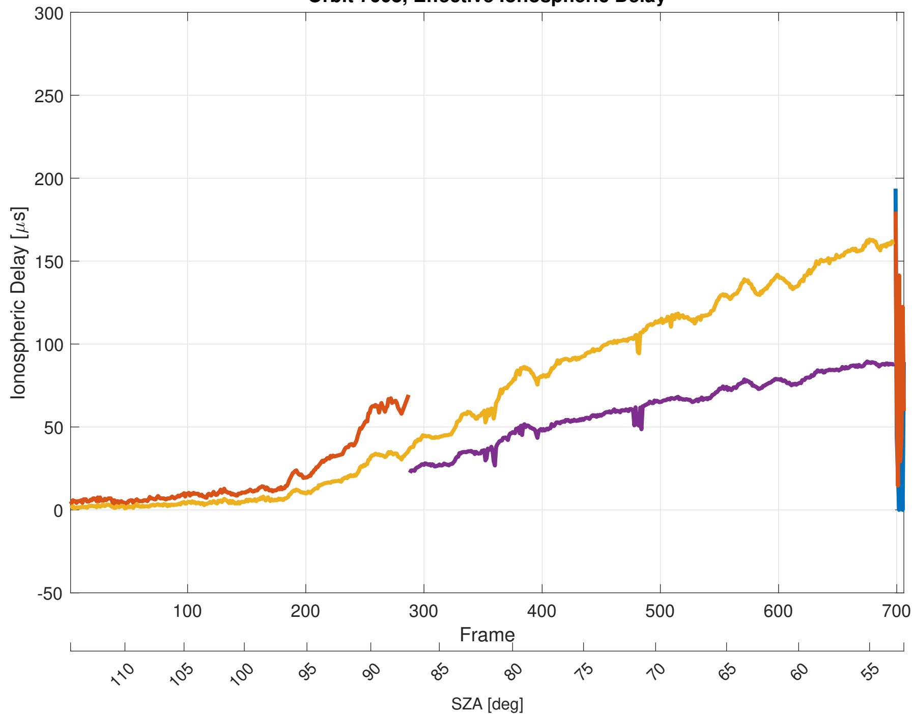
Orbit 7608, Effective Ionospheric Delay
