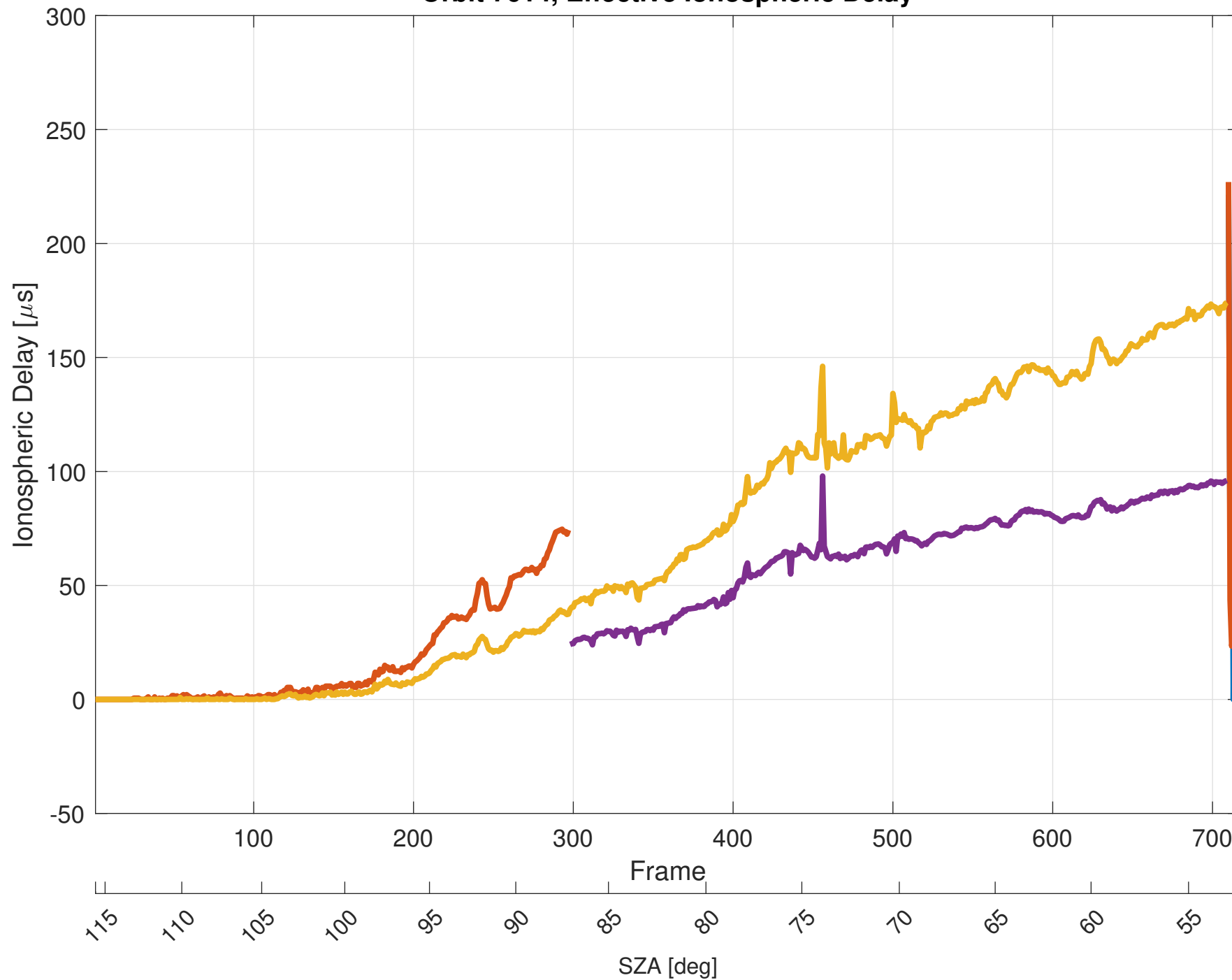
Orbit 7614, Effective Ionospheric Delay
