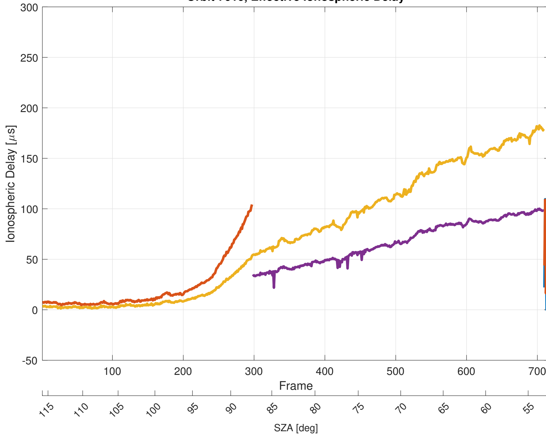
Orbit 7616, Effective Ionospheric Delay
