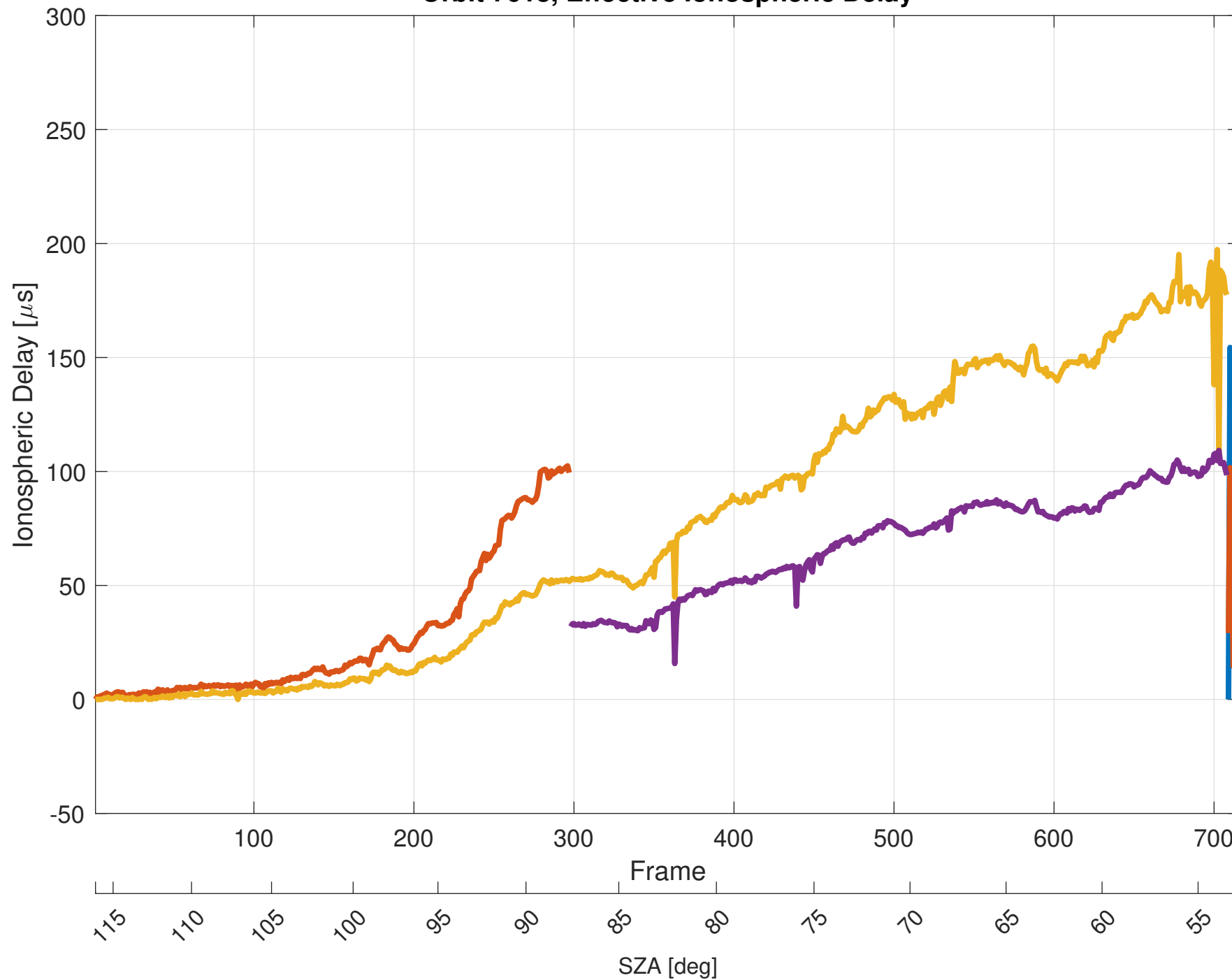
Orbit 7618, Effective Ionospheric Delay
