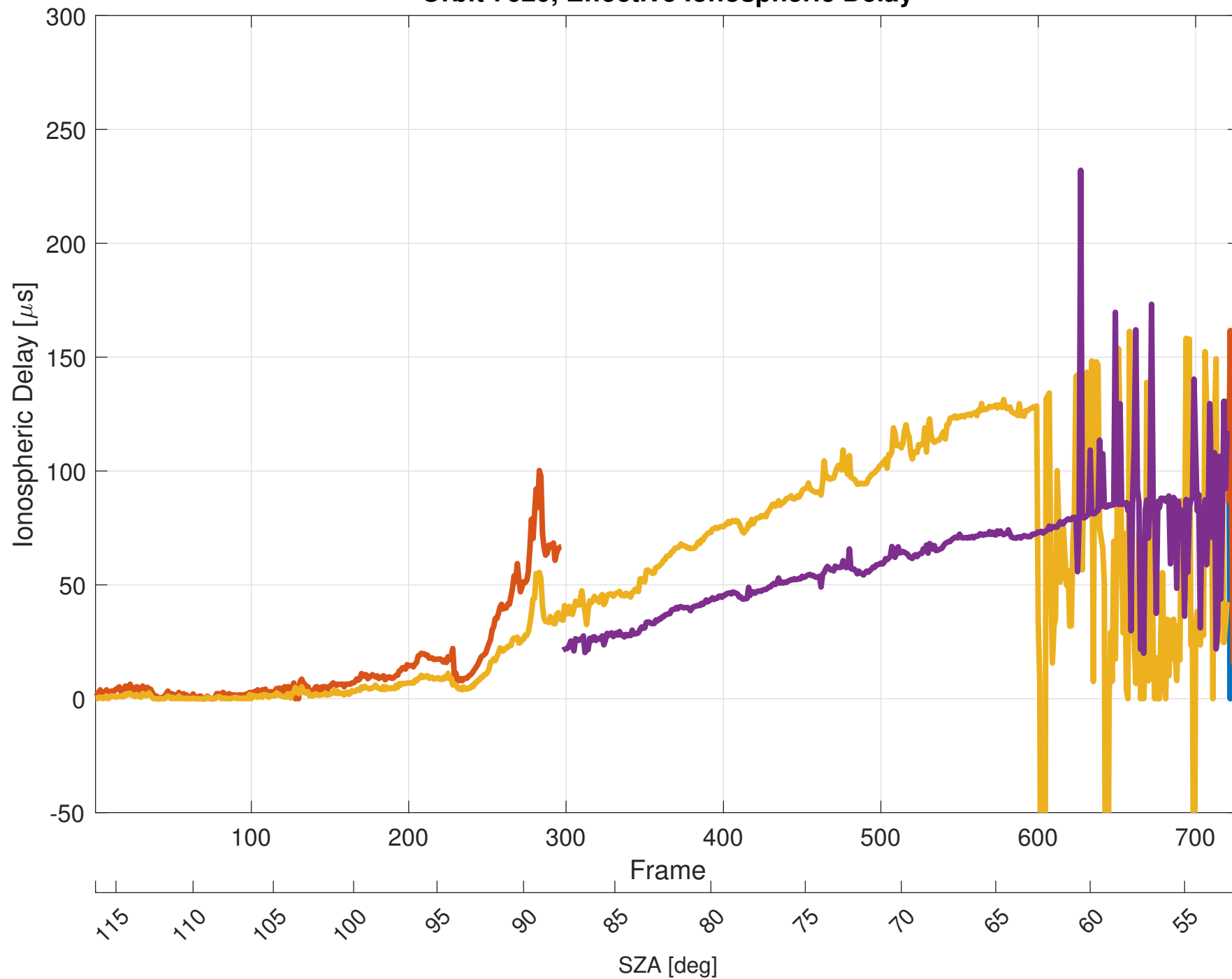
Orbit 7620, Effective Ionospheric Delay
