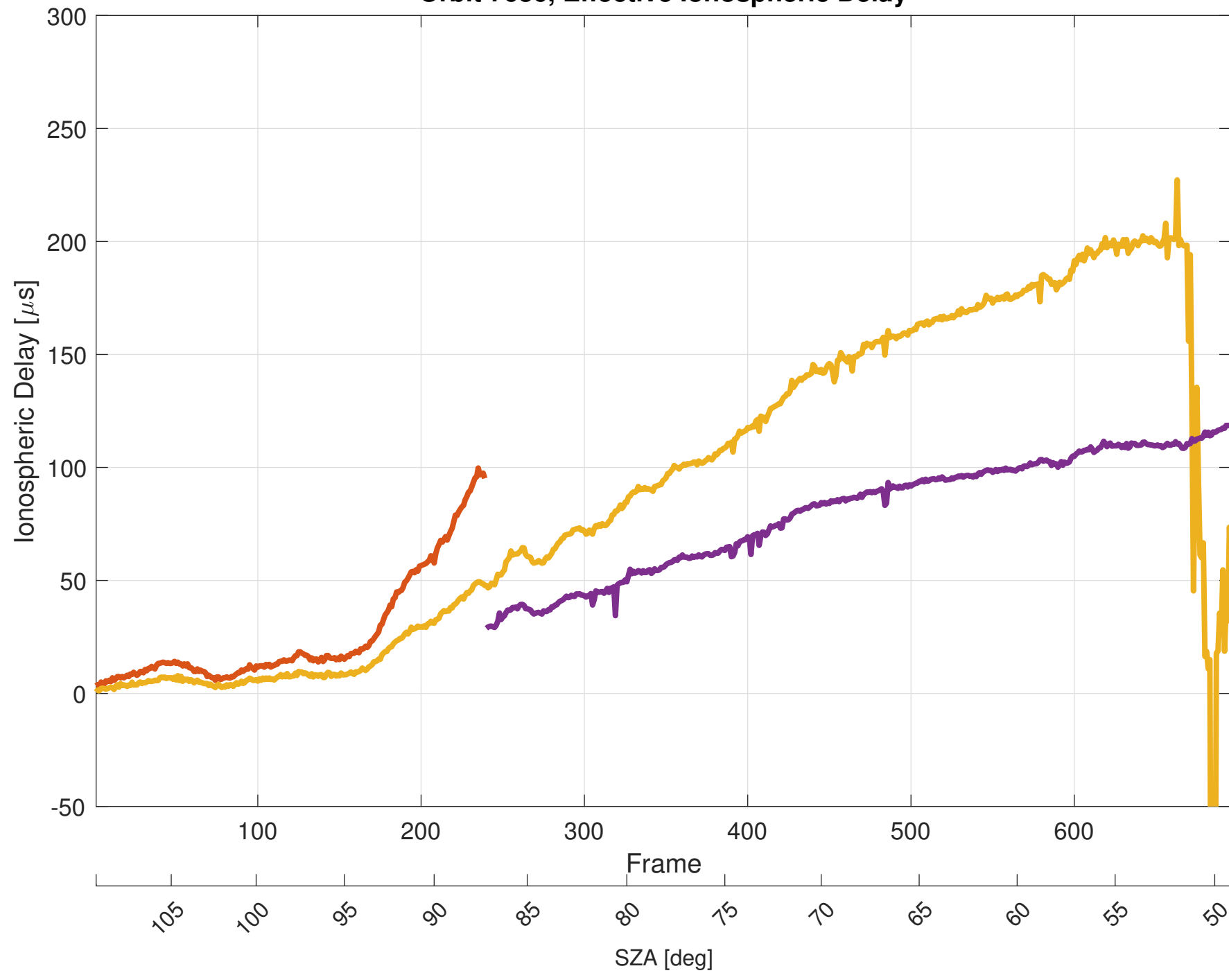
Orbit 7636, Effective Ionospheric Delay
