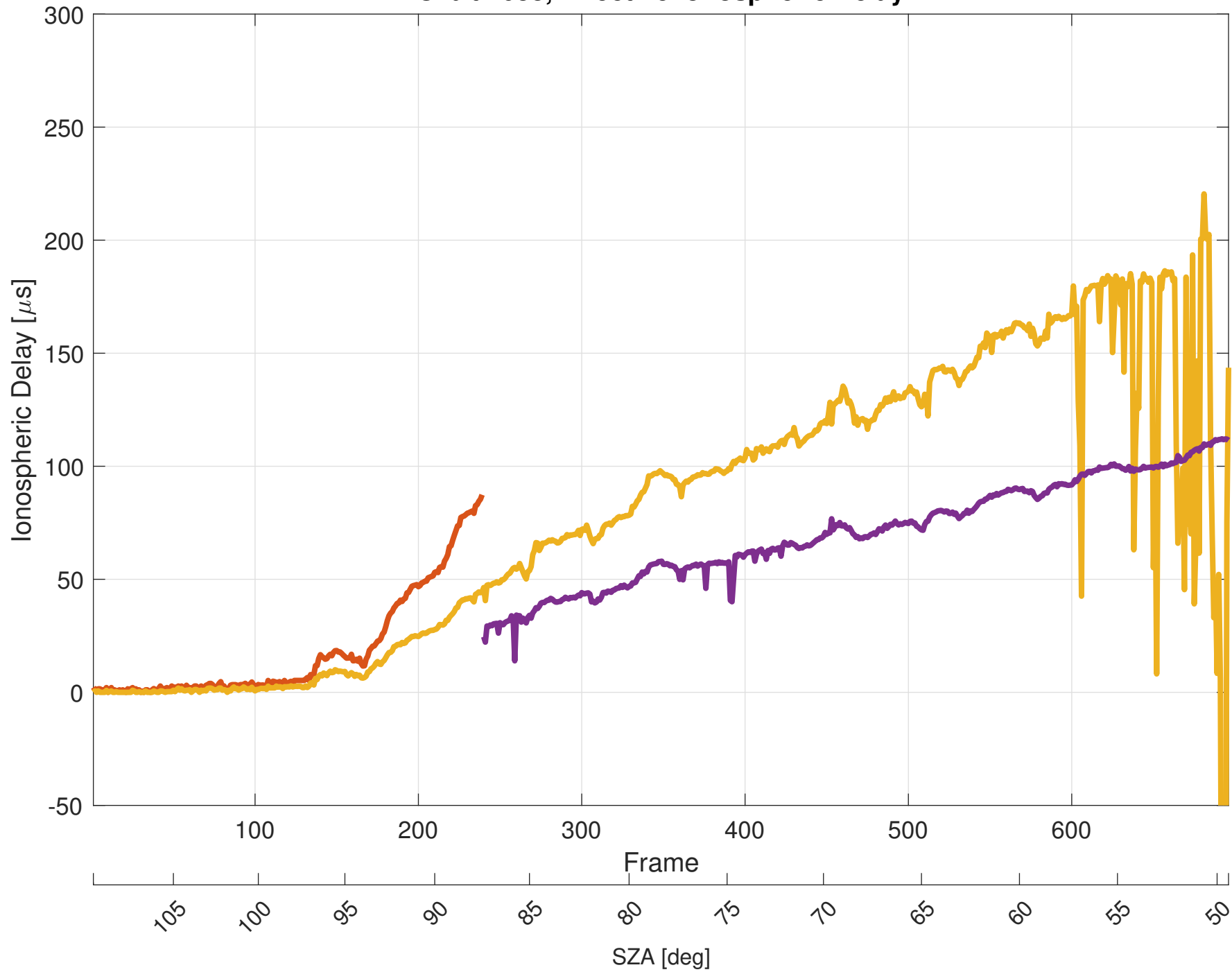
Orbit 7638, Effective Ionospheric Delay
