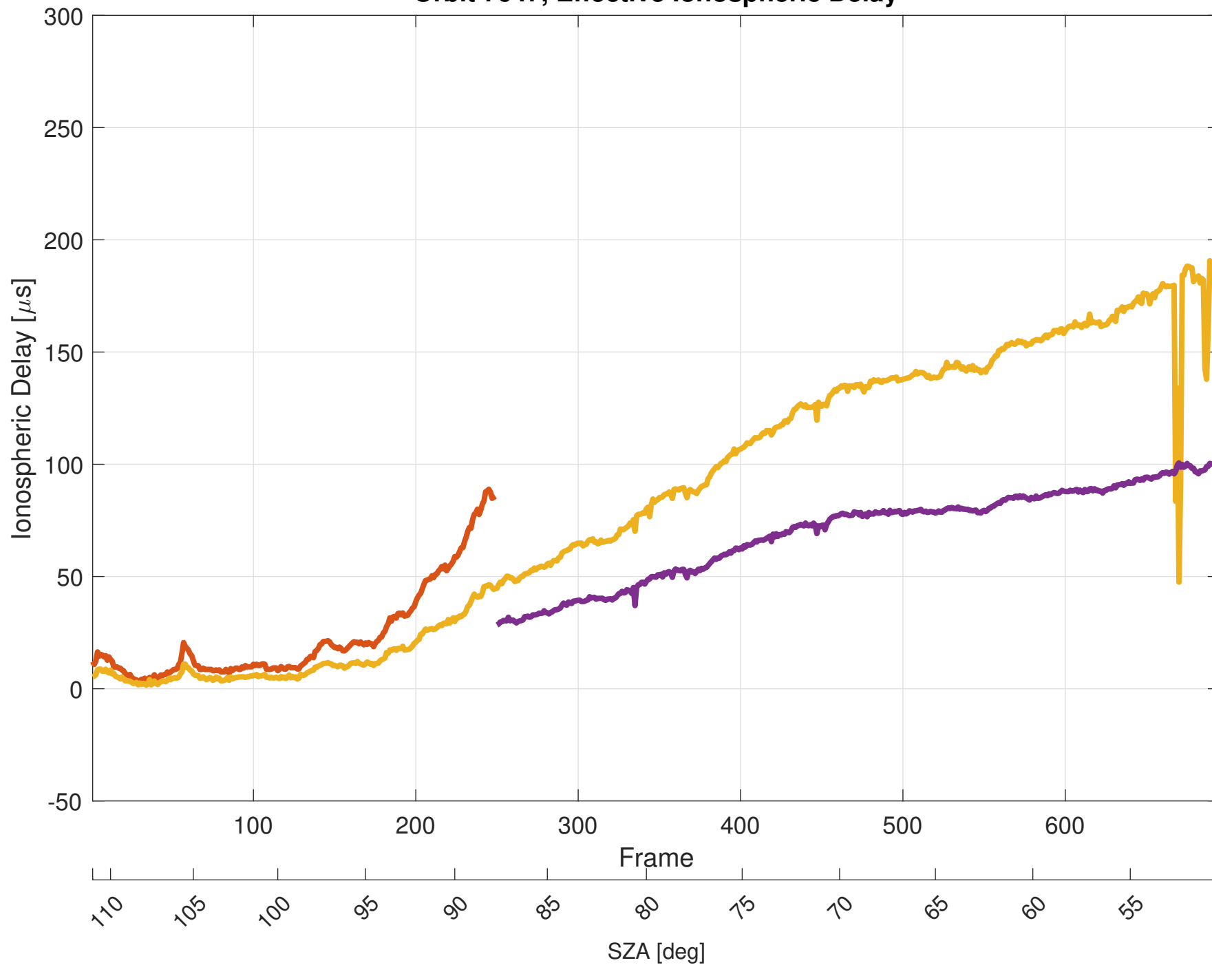
Orbit 7647, Effective Ionospheric Delay
