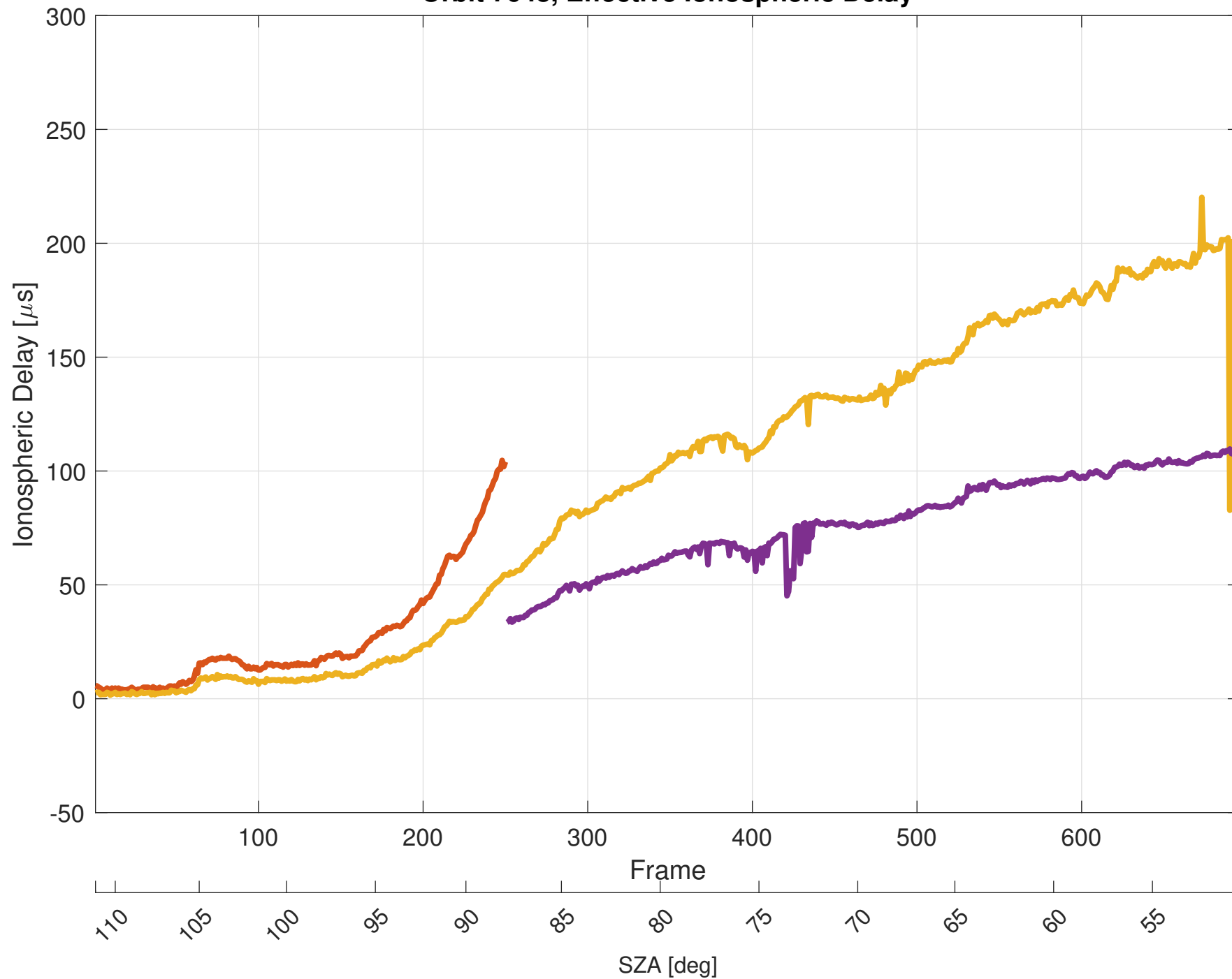
Orbit 7648, Effective Ionospheric Delay
