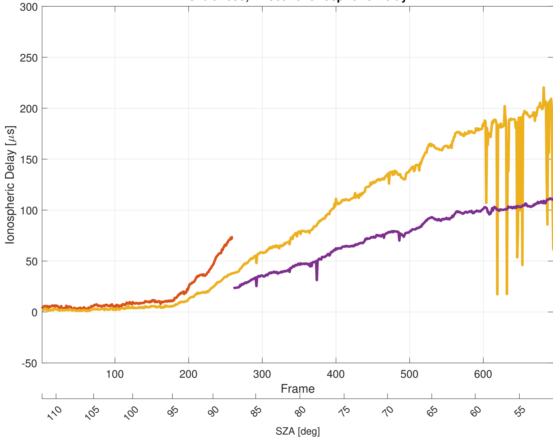
Orbit 7653, Effective Ionospheric Delay
