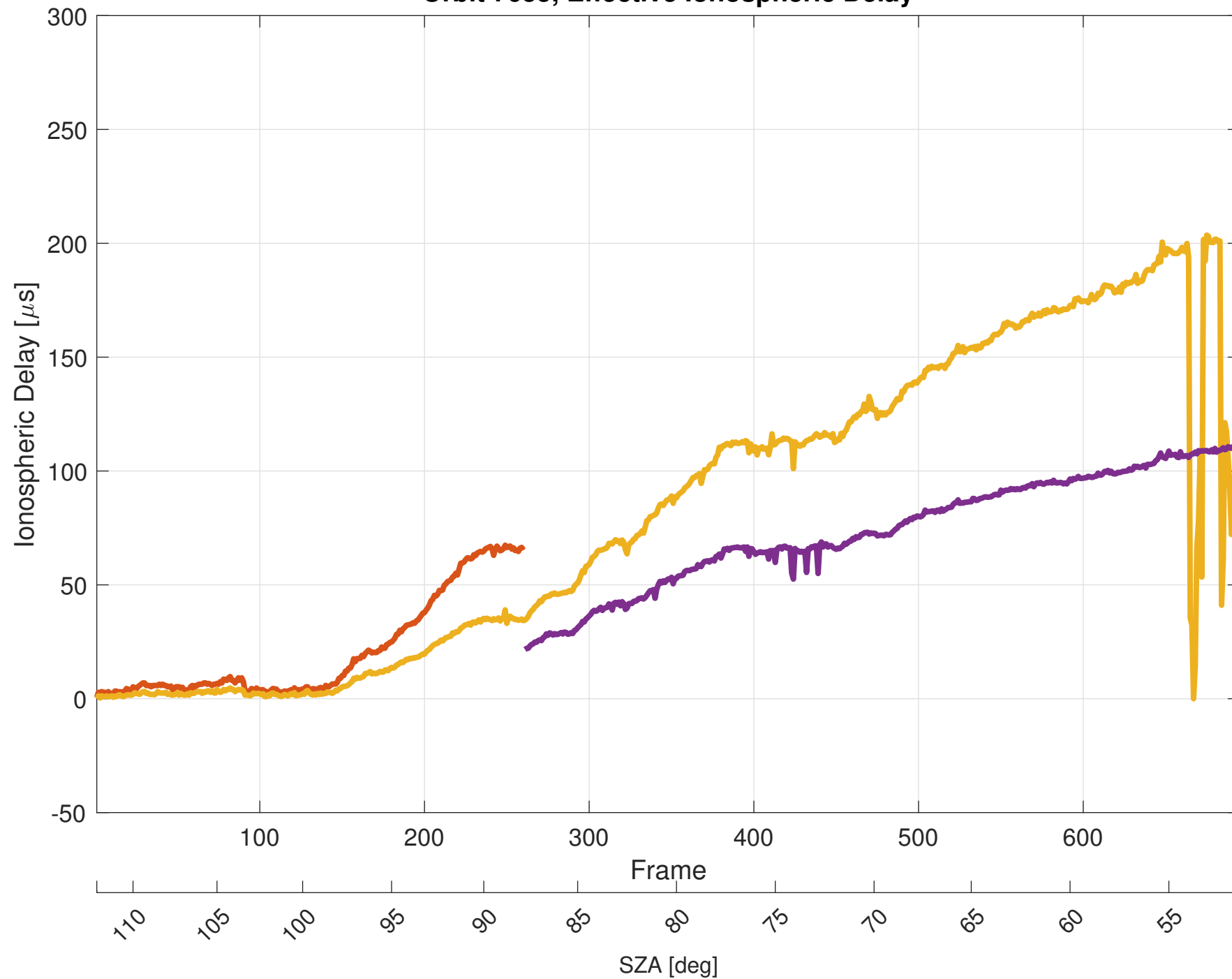
Orbit 7655, Effective Ionospheric Delay
