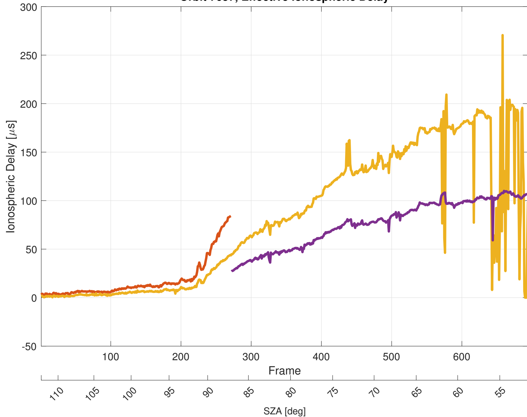
Orbit 7657, Effective Ionospheric Delay
