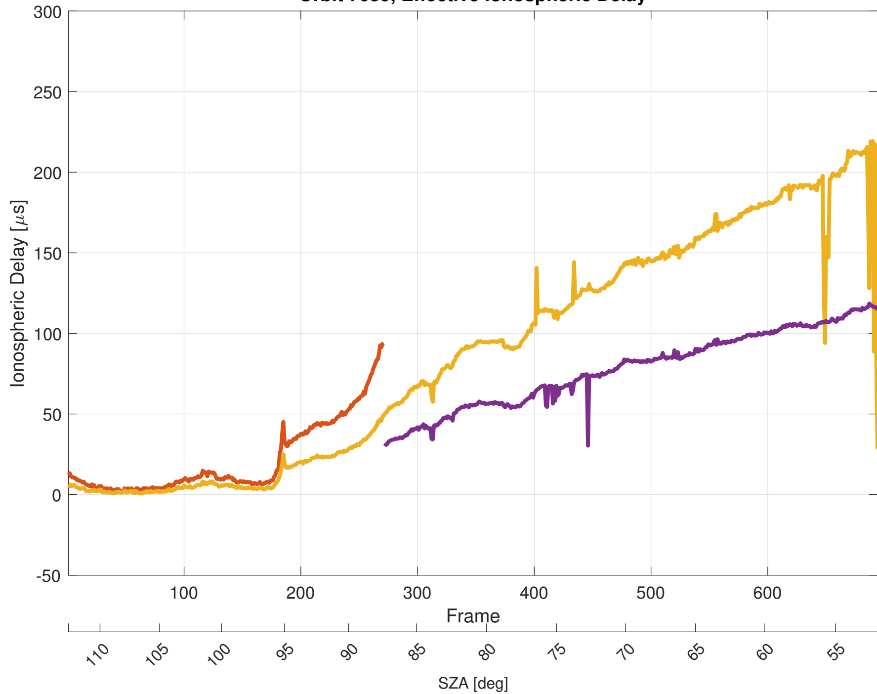
Orbit 7659, Effective Ionospheric Delay
