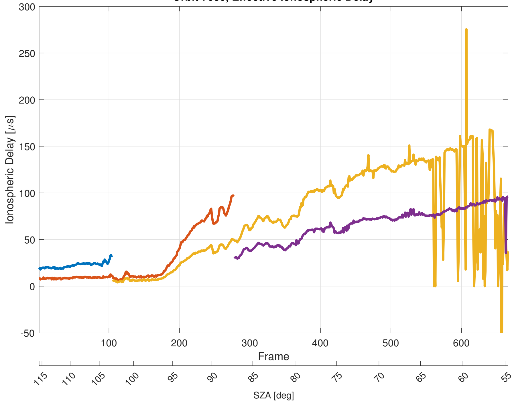
Orbit 7680, Effective Ionospheric Delay
