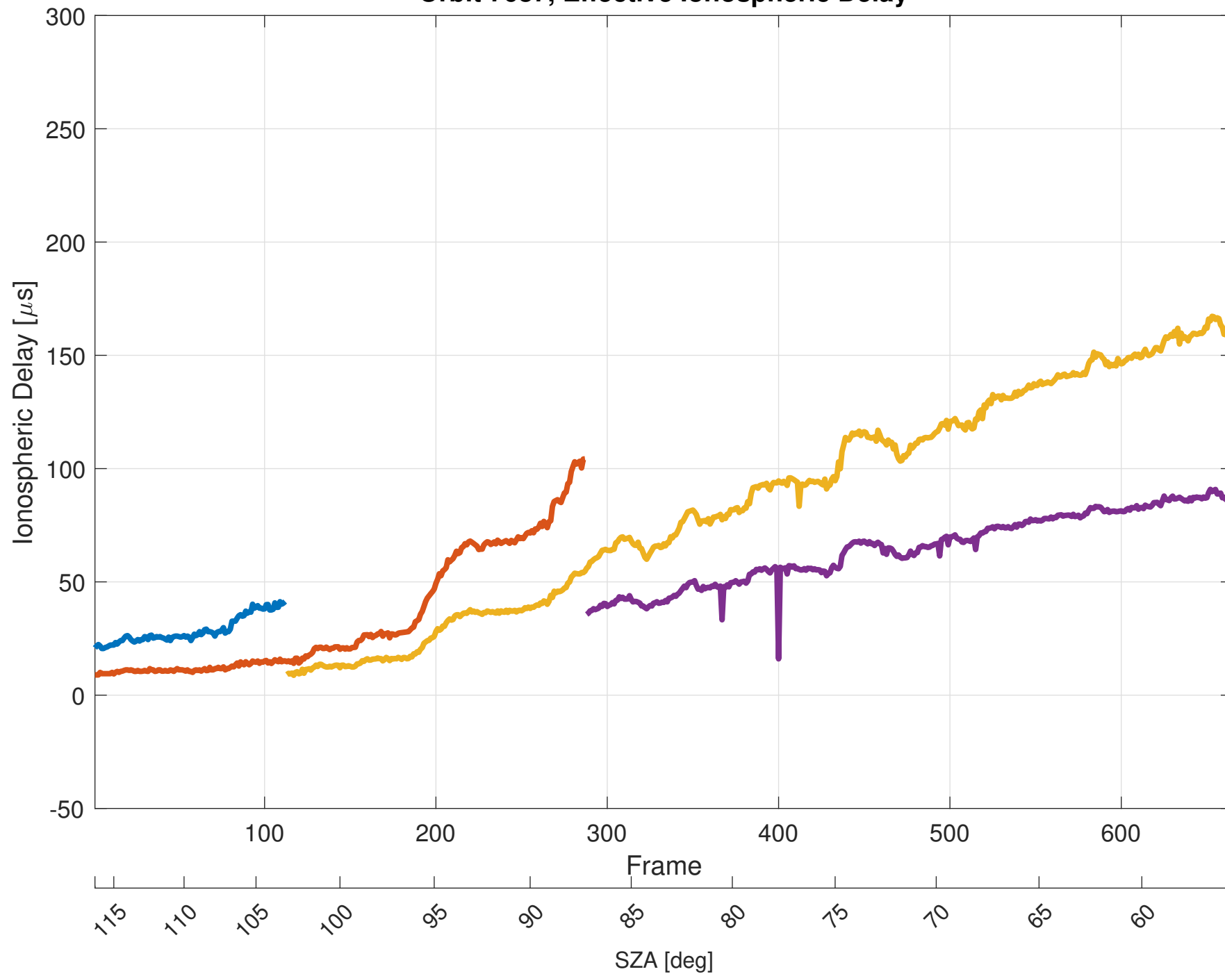
Orbit 7687, Effective Ionospheric Delay
