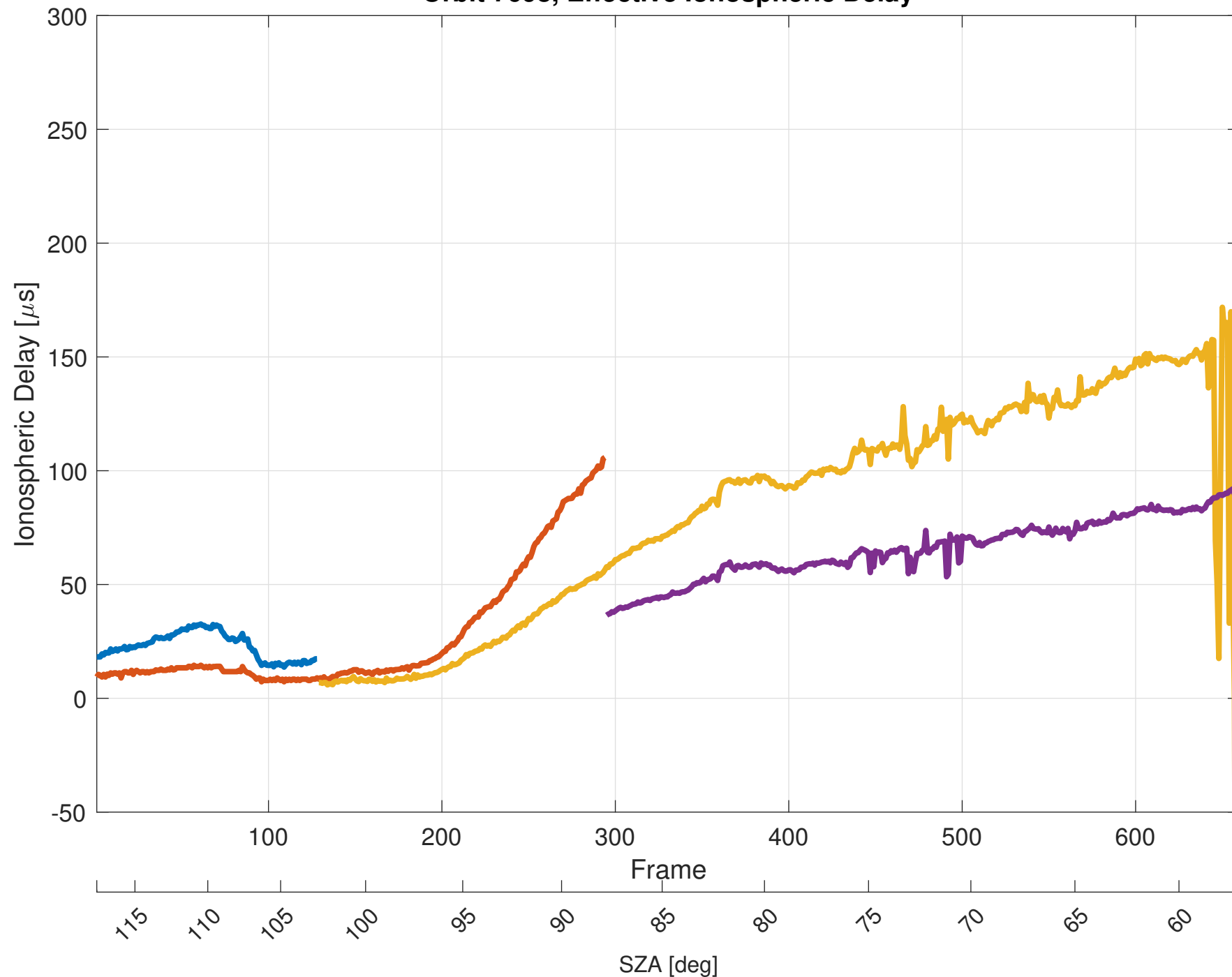
Orbit 7698, Effective Ionospheric Delay
