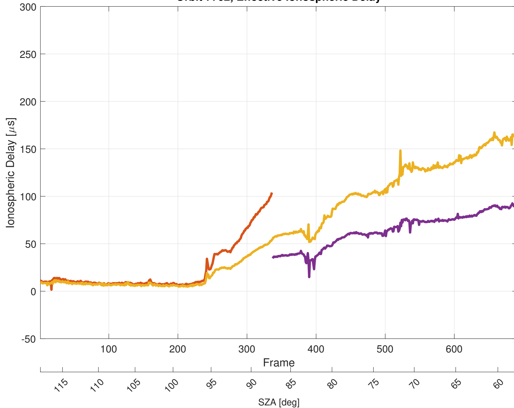
Orbit 7702, Effective Ionospheric Delay
