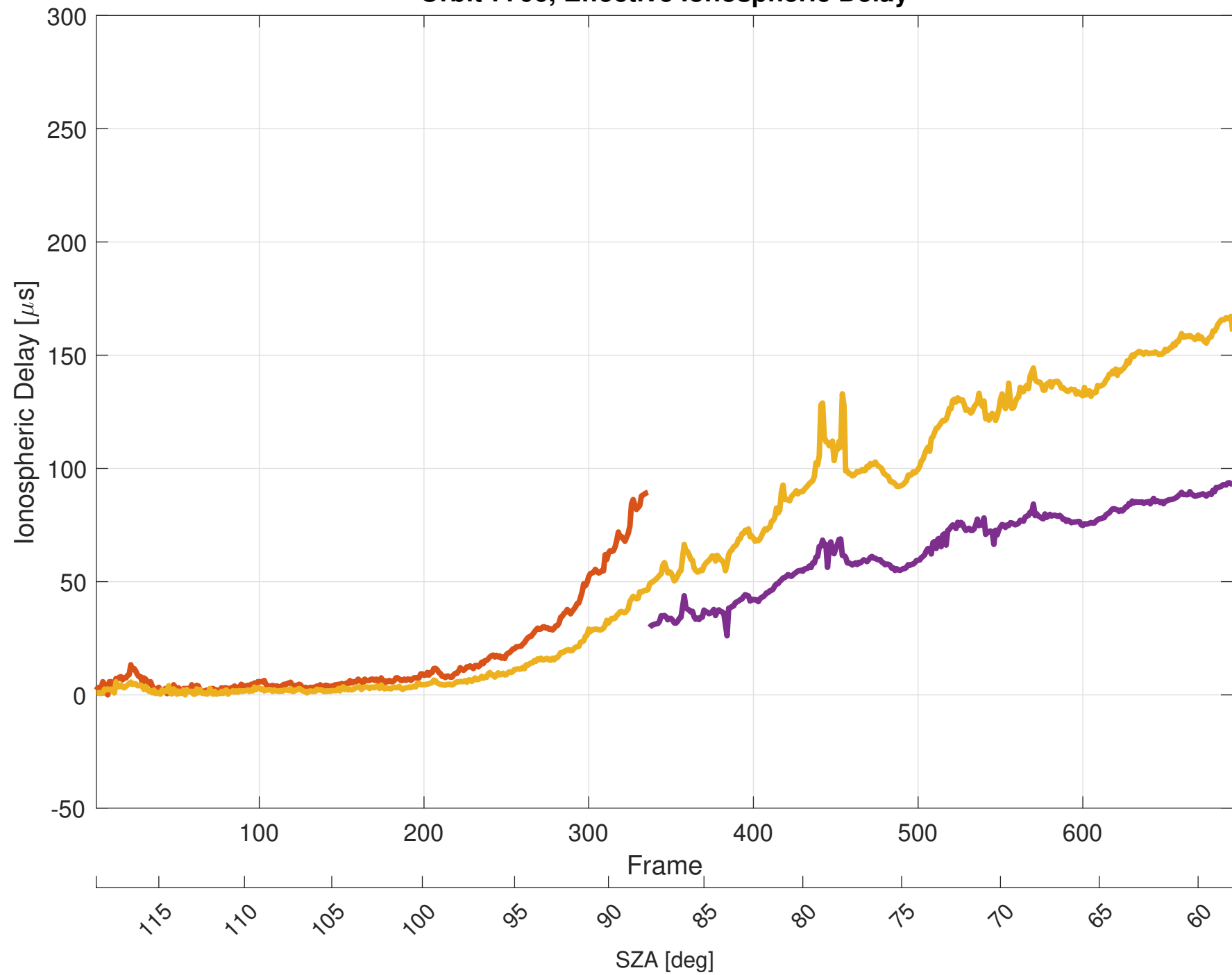
Orbit 7706, Effective Ionospheric Delay
