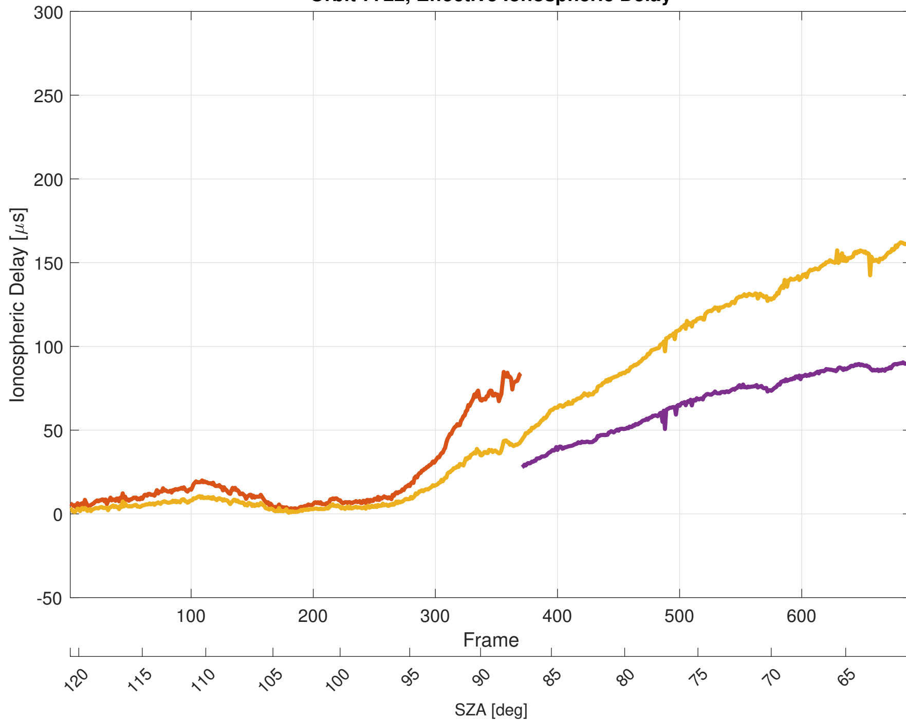
Orbit 7722, Effective Ionospheric Delay
