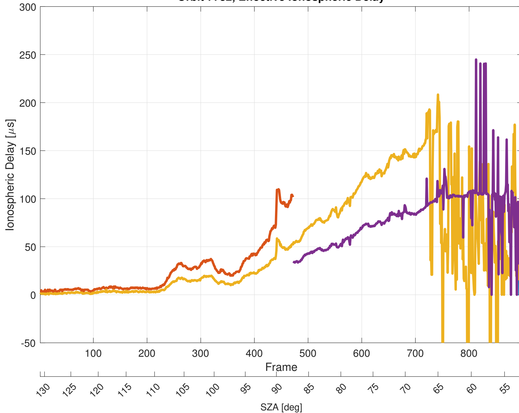
Orbit 7732, Effective Ionospheric Delay
