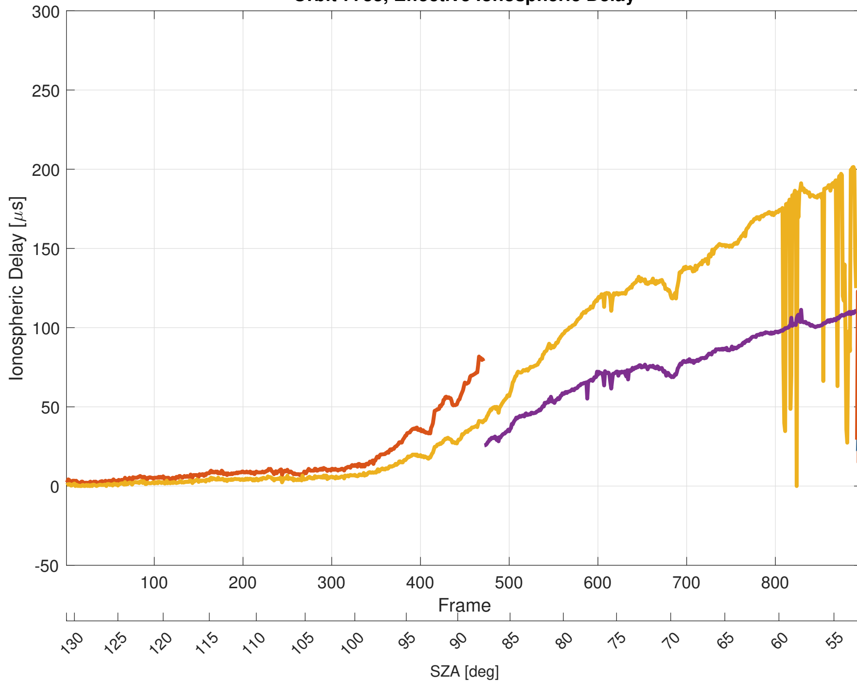
Orbit 7733, Effective Ionospheric Delay
