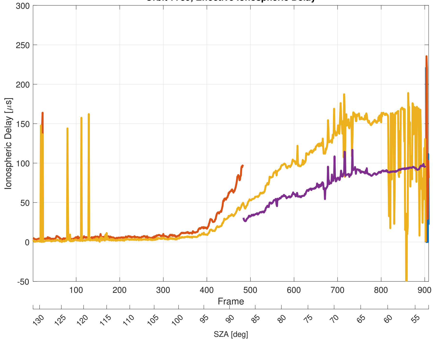
Orbit 7739, Effective Ionospheric Delay
