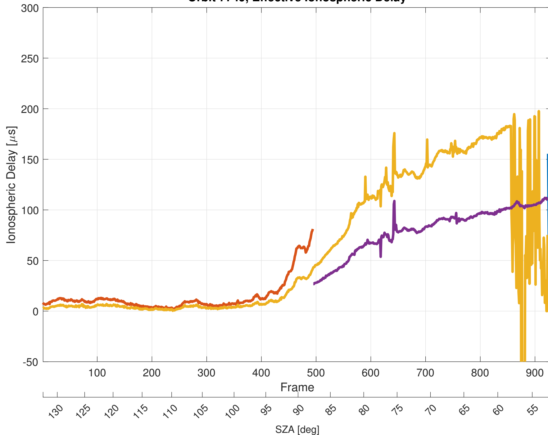
Orbit 7749, Effective Ionospheric Delay
