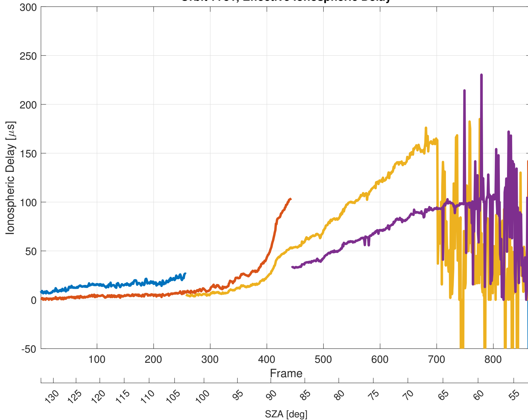
Orbit 7751, Effective Ionospheric Delay
