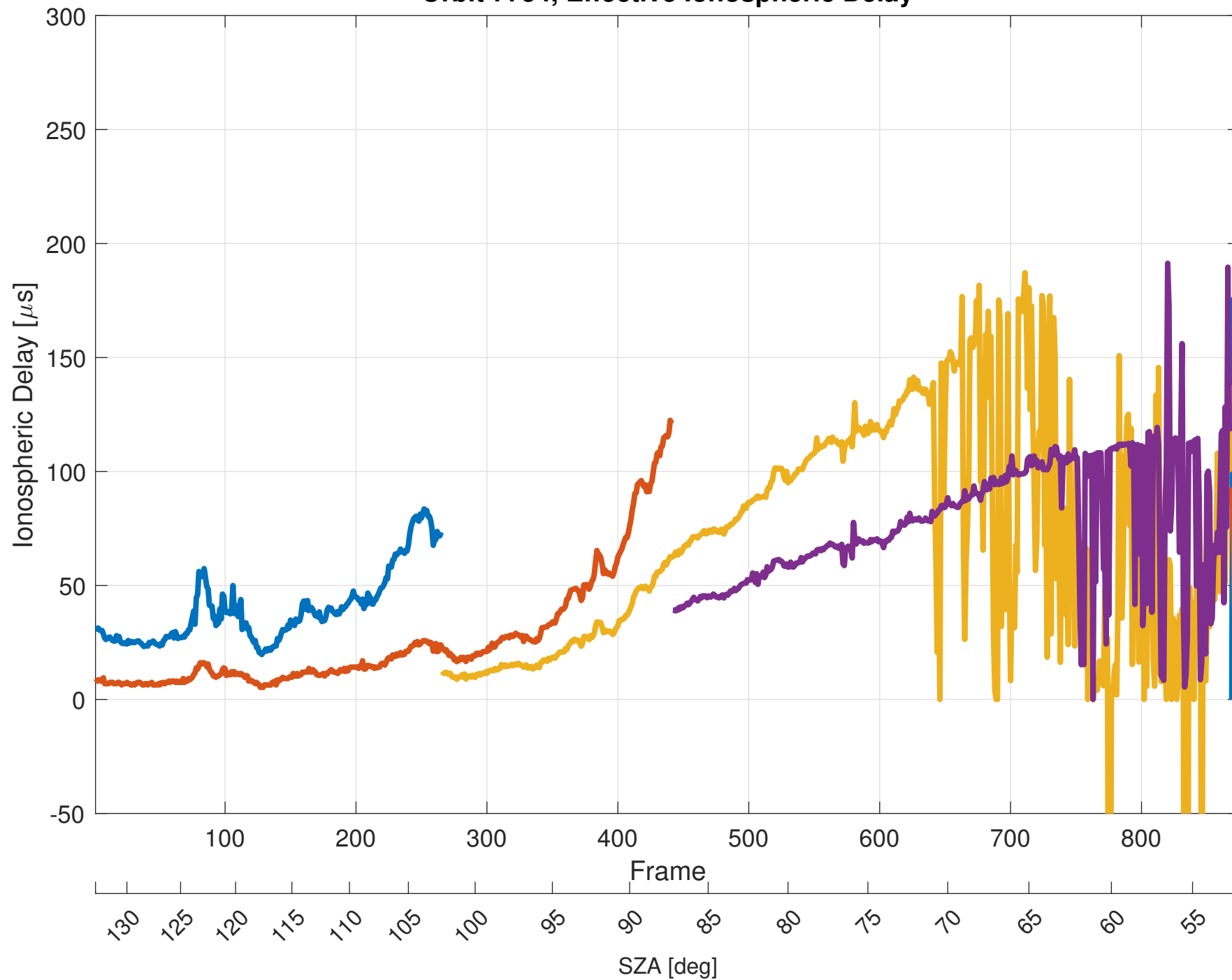
Orbit 7754, Effective Ionospheric Delay
