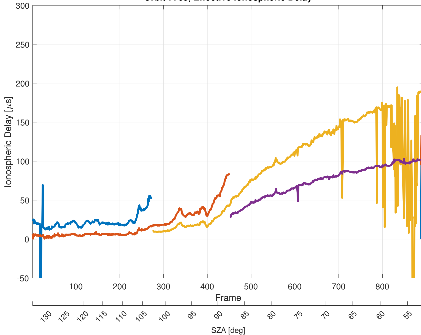
Orbit 7765, Effective Ionospheric Delay
