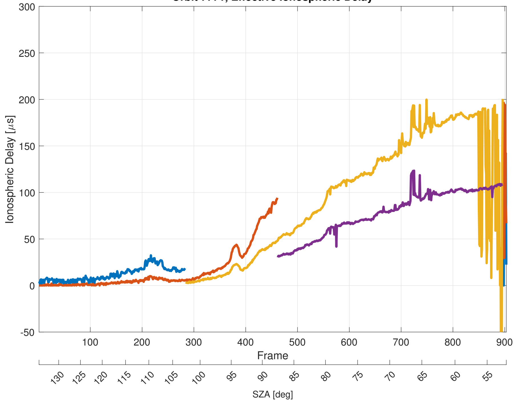
Orbit 7771, Effective Ionospheric Delay
