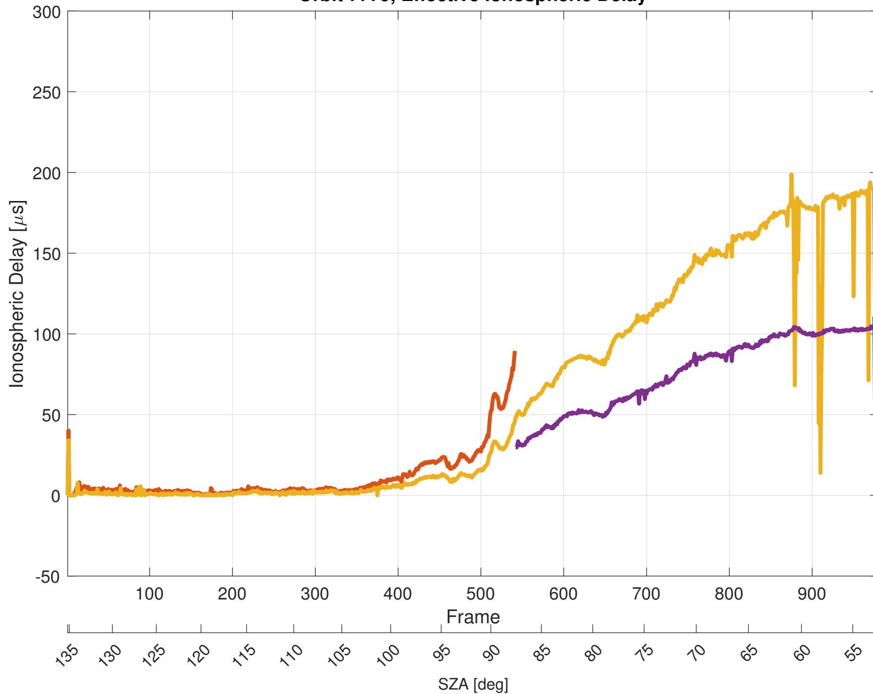
Orbit 7779, Effective Ionospheric Delay
