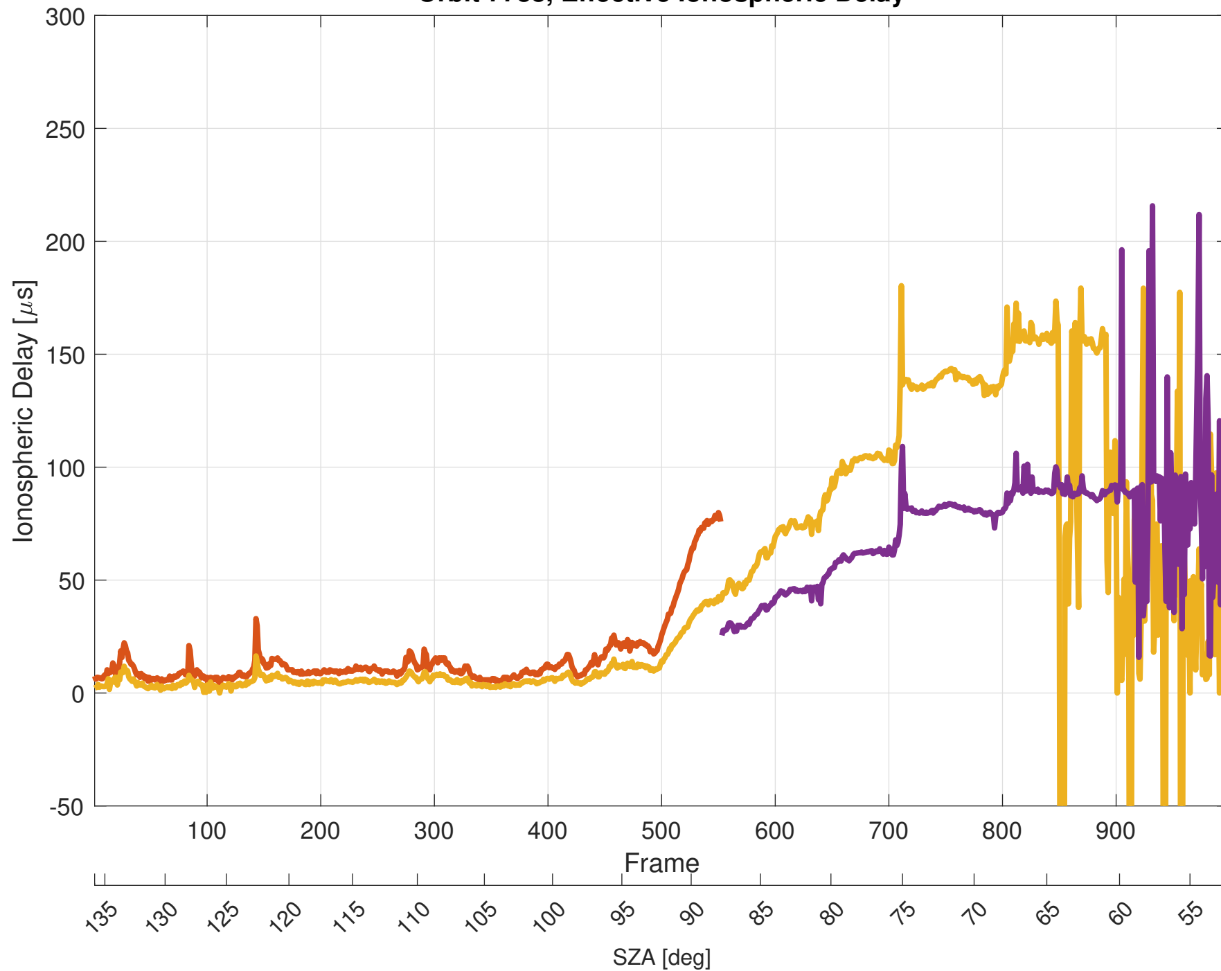
Orbit 7788, Effective Ionospheric Delay
