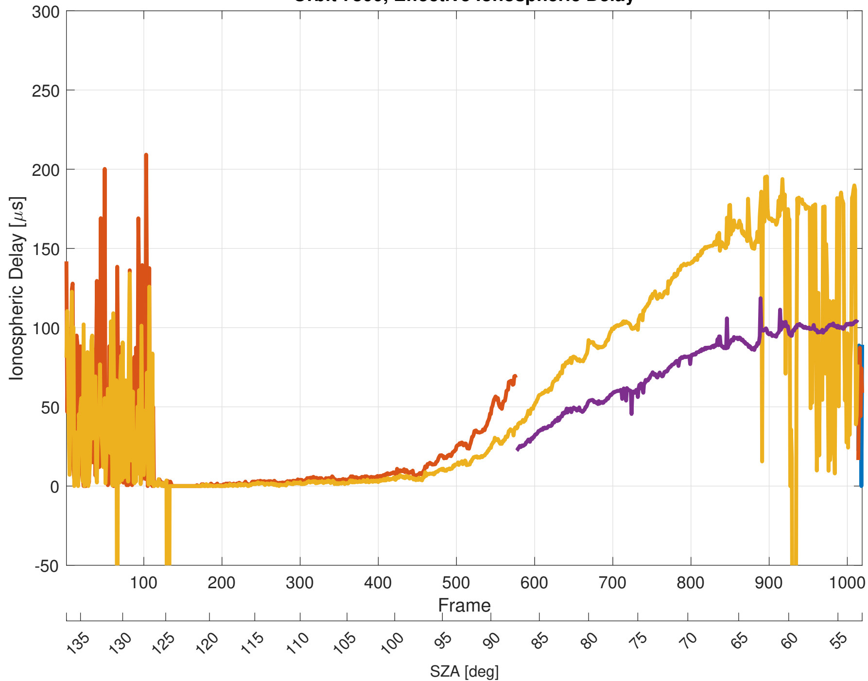
Orbit 7800, Effective Ionospheric Delay
