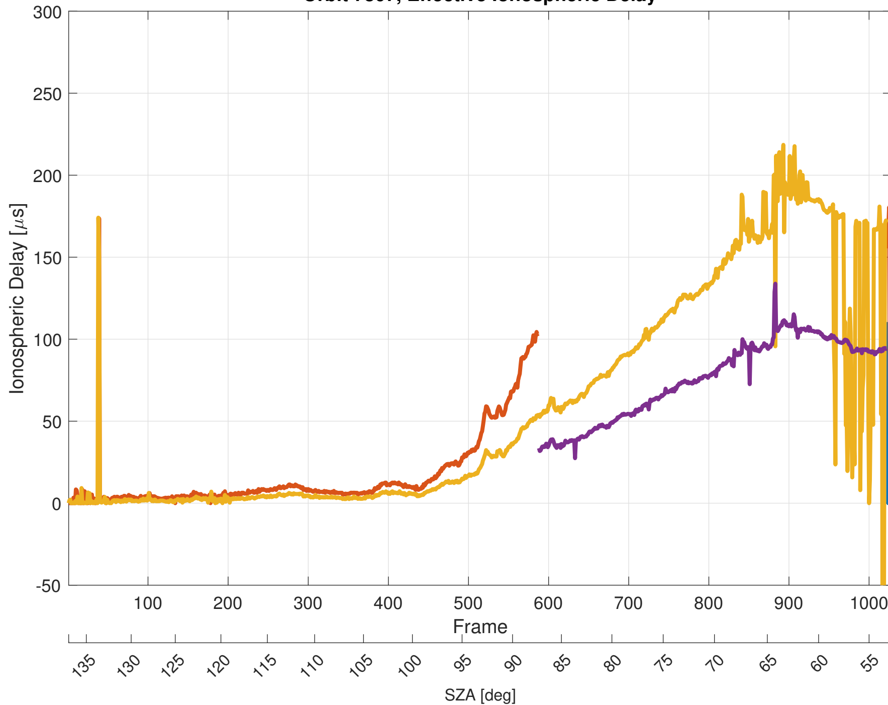
Orbit 7807, Effective Ionospheric Delay
