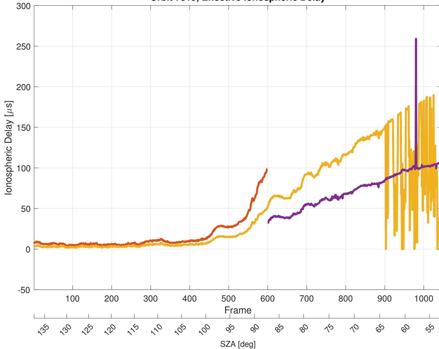
Orbit 7815, Effective Ionospheric Delay
