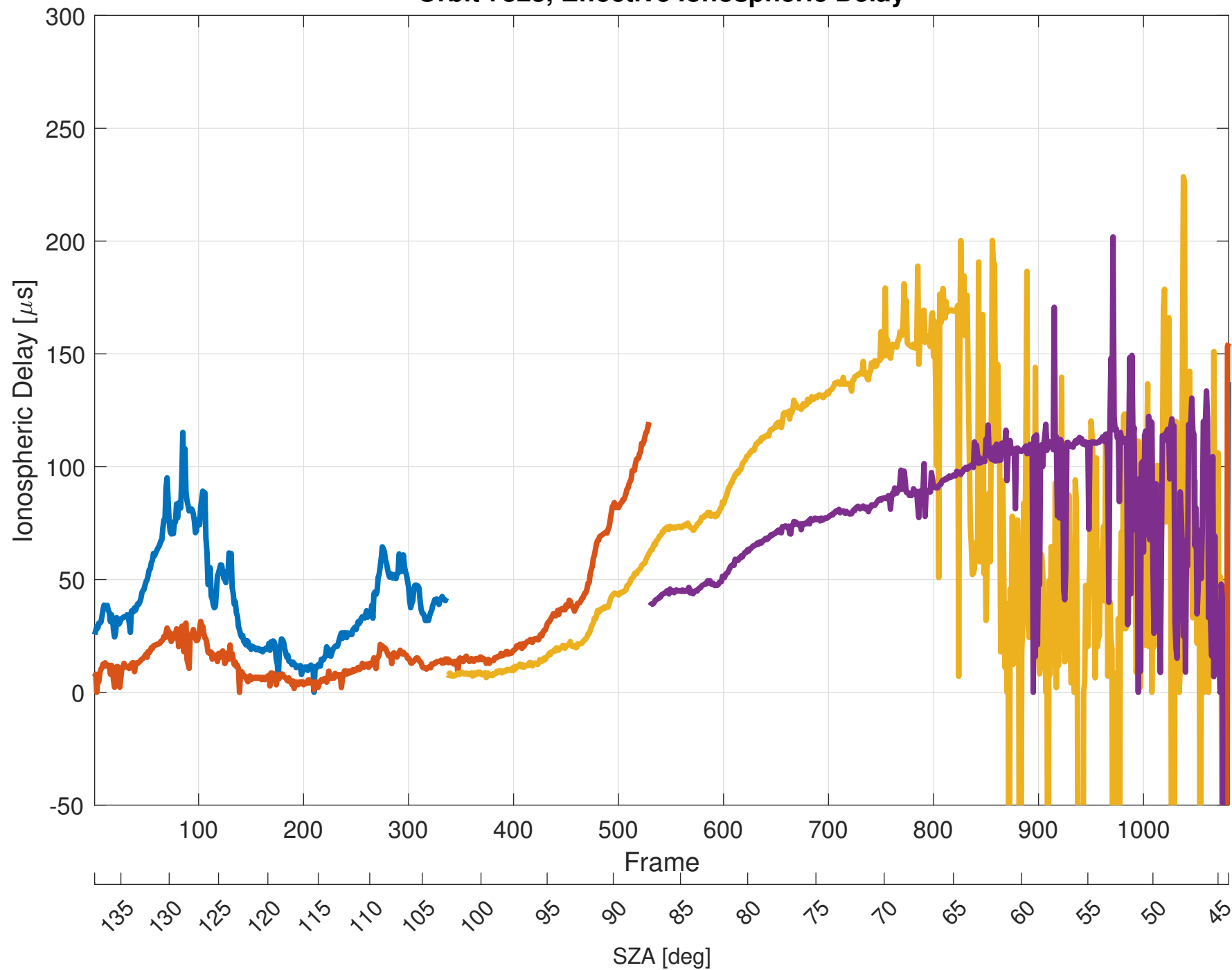
Orbit 7823, Effective Ionospheric Delay
