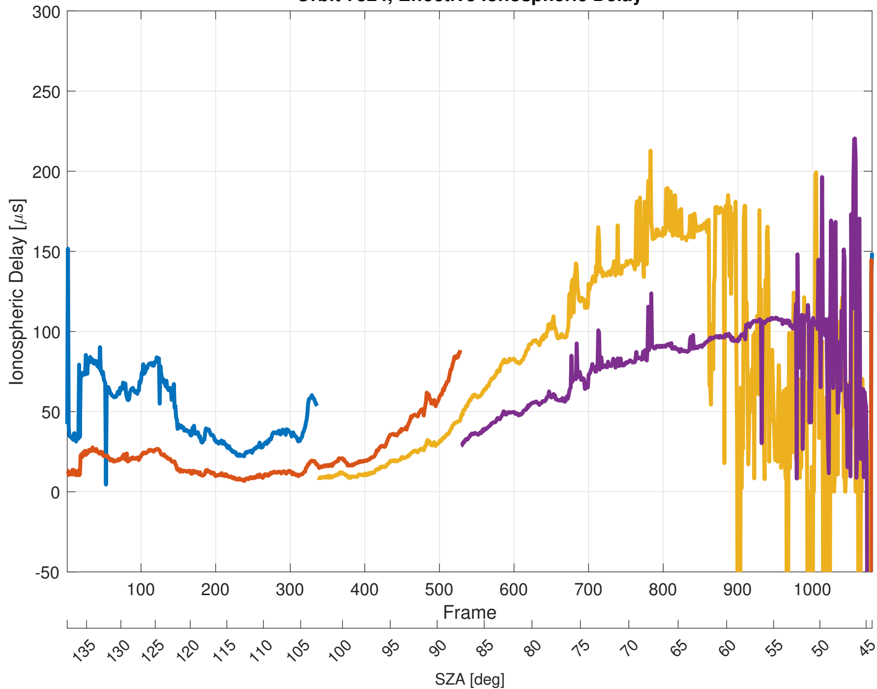
Orbit 7824, Effective Ionospheric Delay
