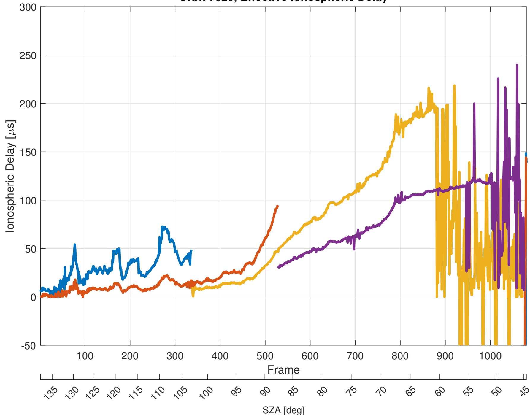
Orbit 7825, Effective Ionospheric Delay
