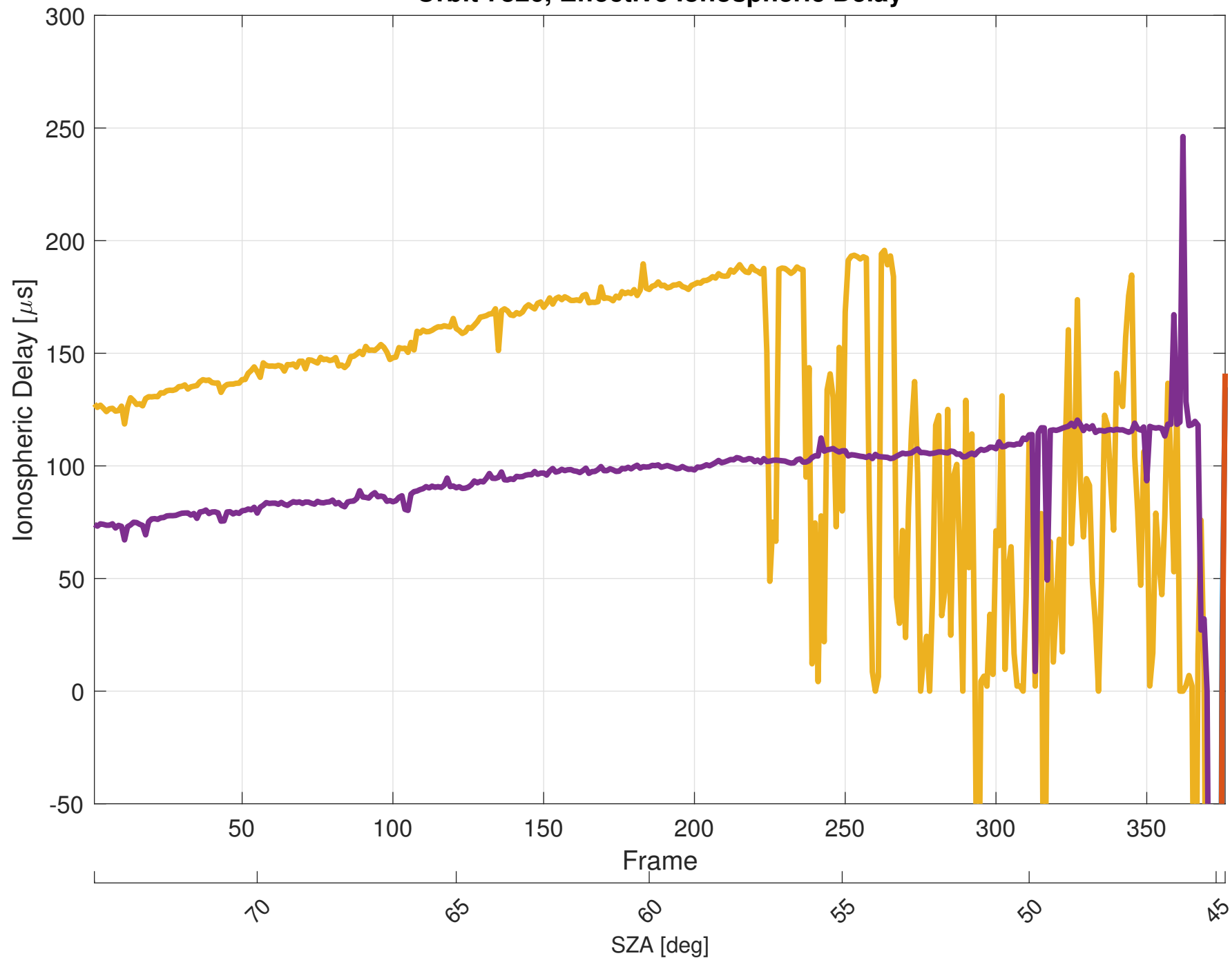
Orbit 7826, Effective Ionospheric Delay
