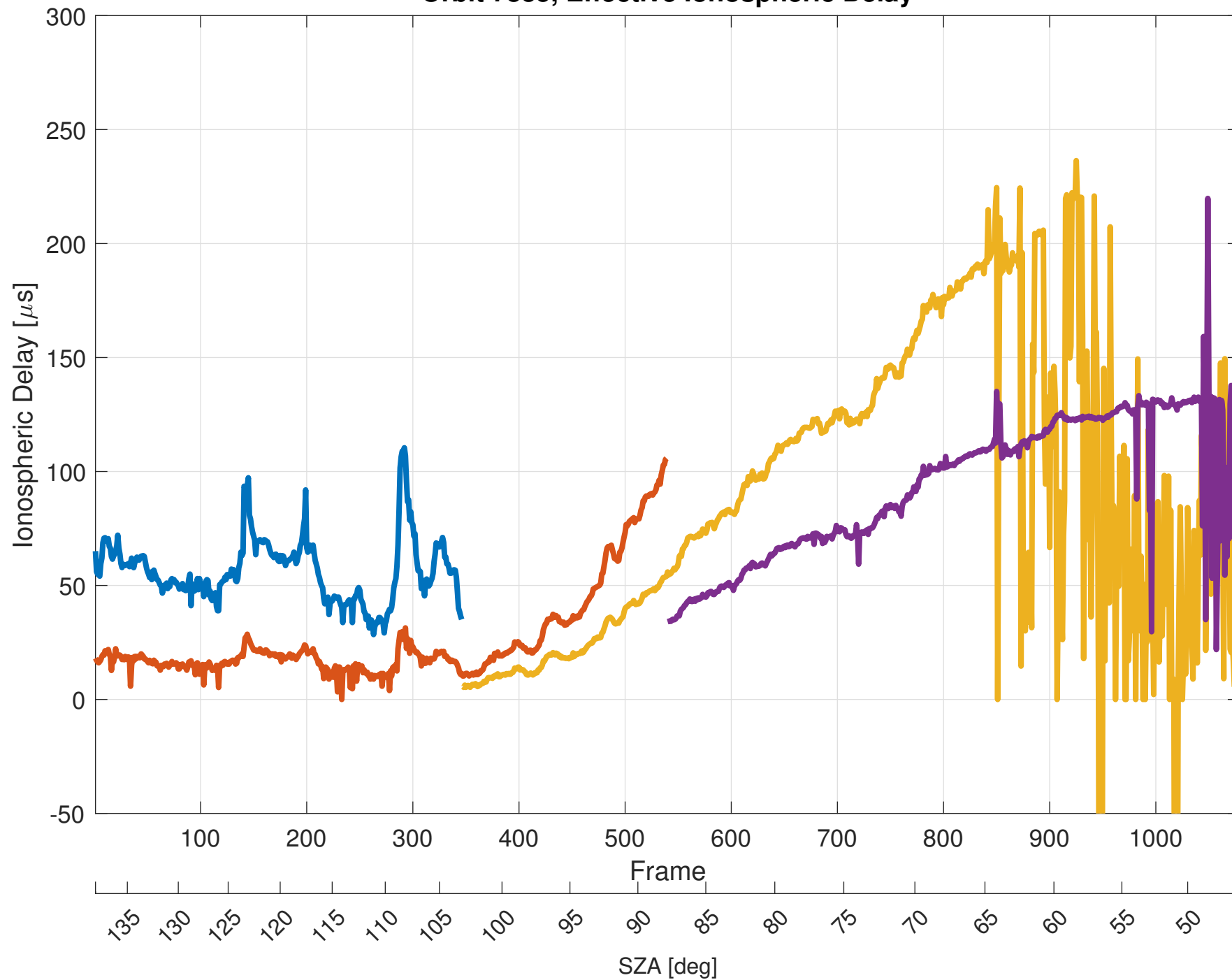
Orbit 7835, Effective Ionospheric Delay
