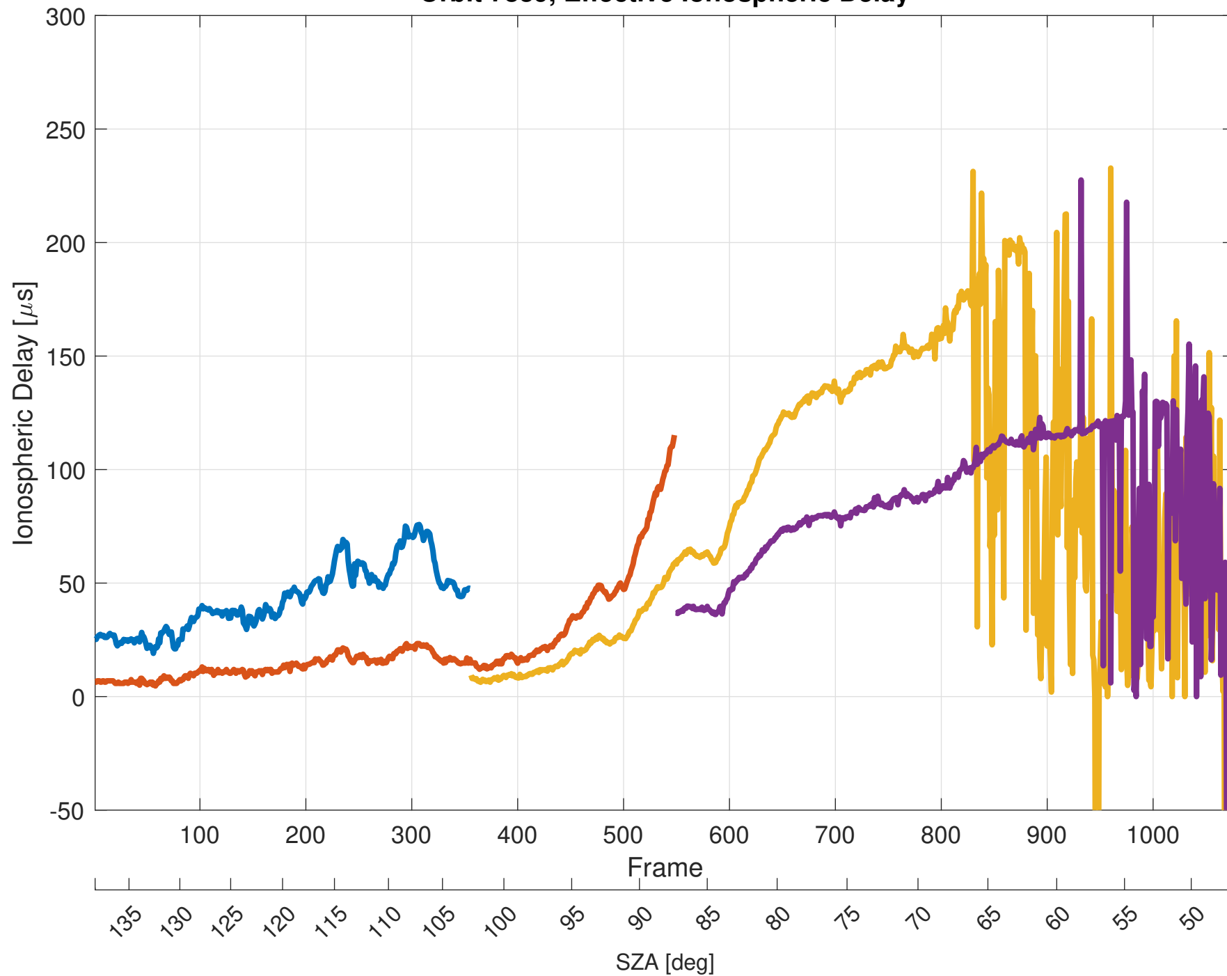
Orbit 7839, Effective Ionospheric Delay
