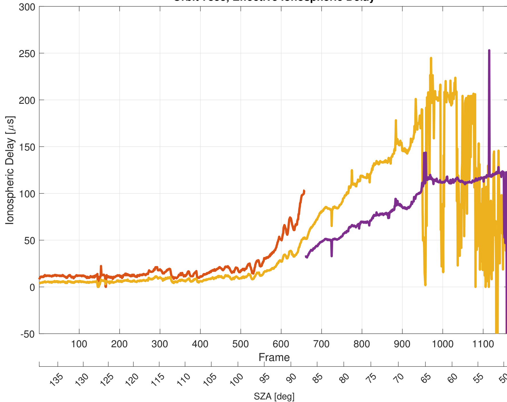
Orbit 7853, Effective Ionospheric Delay
