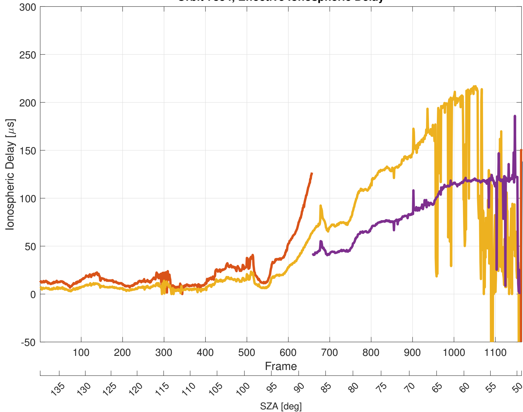
Orbit 7854, Effective Ionospheric Delay
