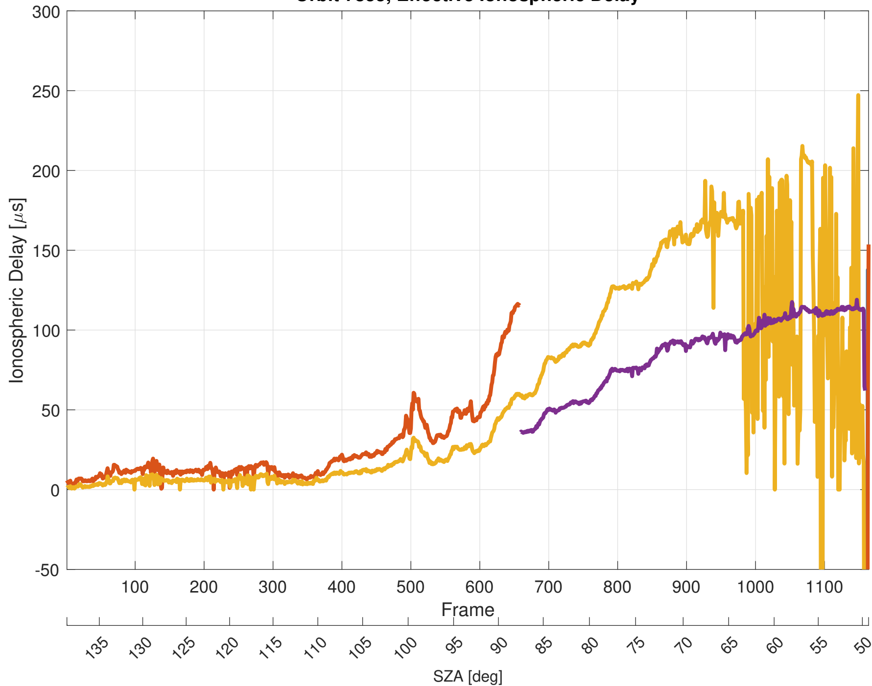
Orbit 7855, Effective Ionospheric Delay
