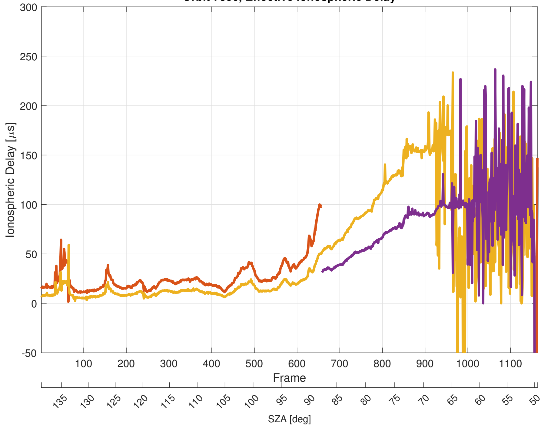
Orbit 7856, Effective Ionospheric Delay
