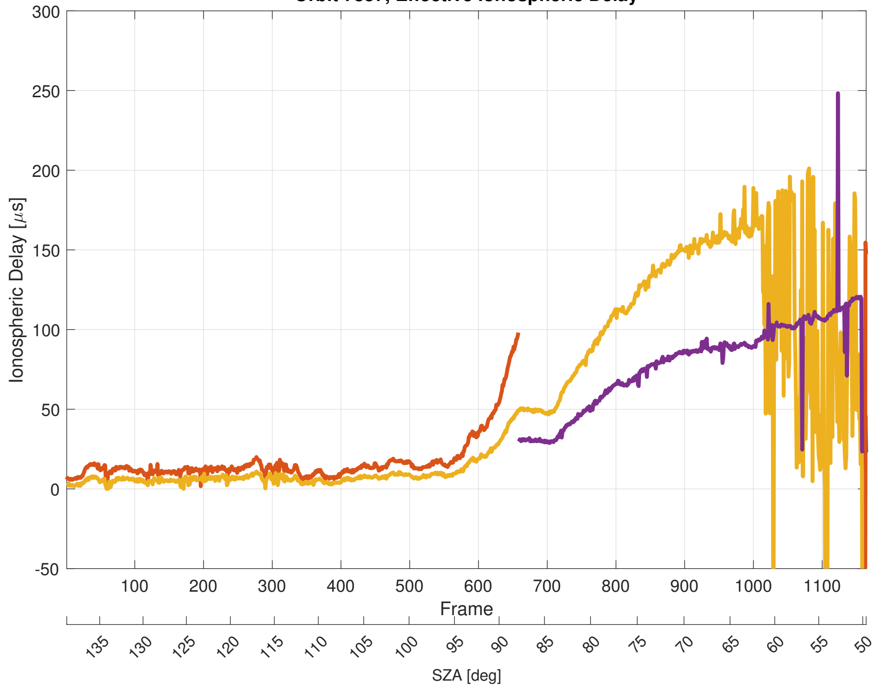
Orbit 7857, Effective Ionospheric Delay
