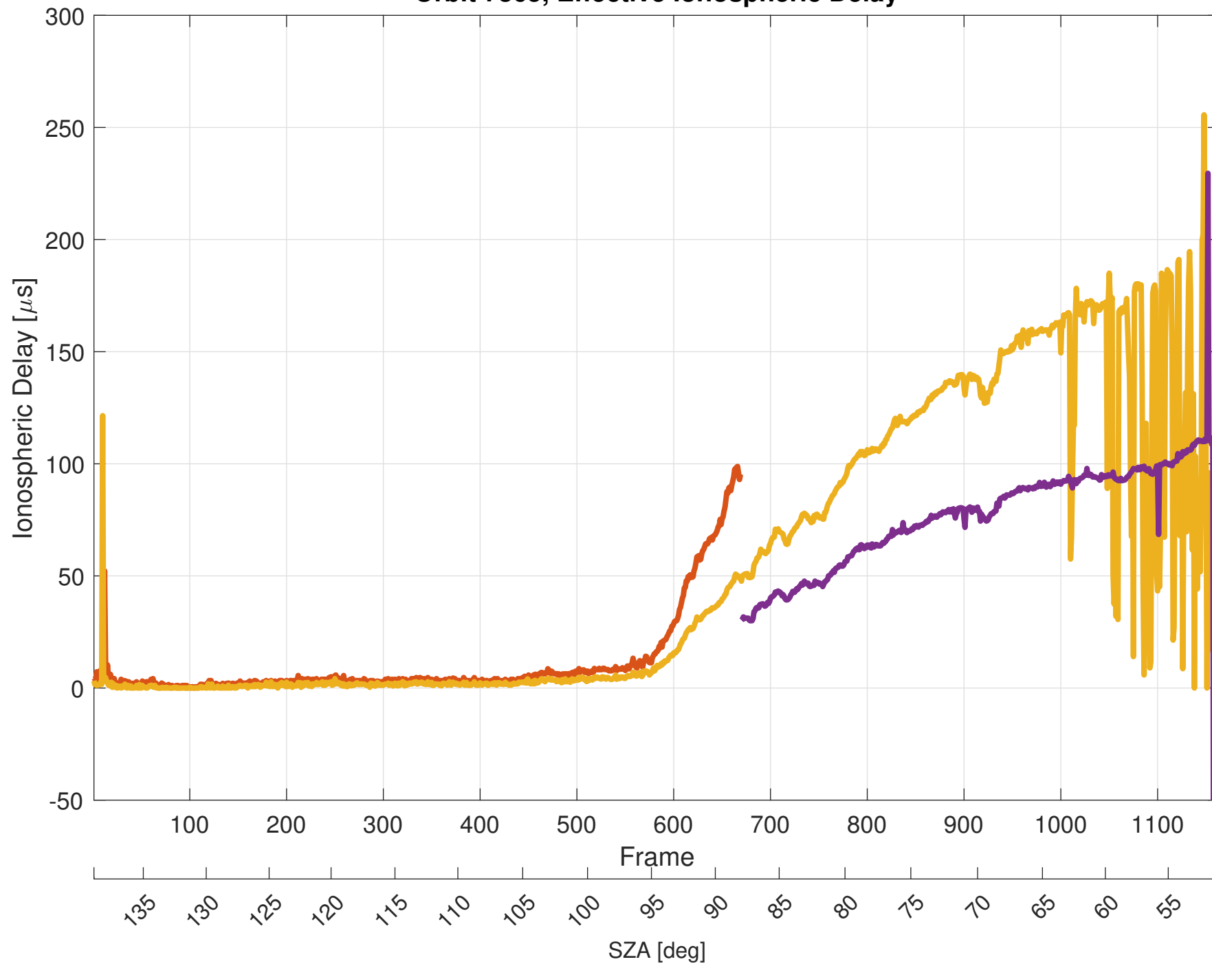
Orbit 7865, Effective Ionospheric Delay
