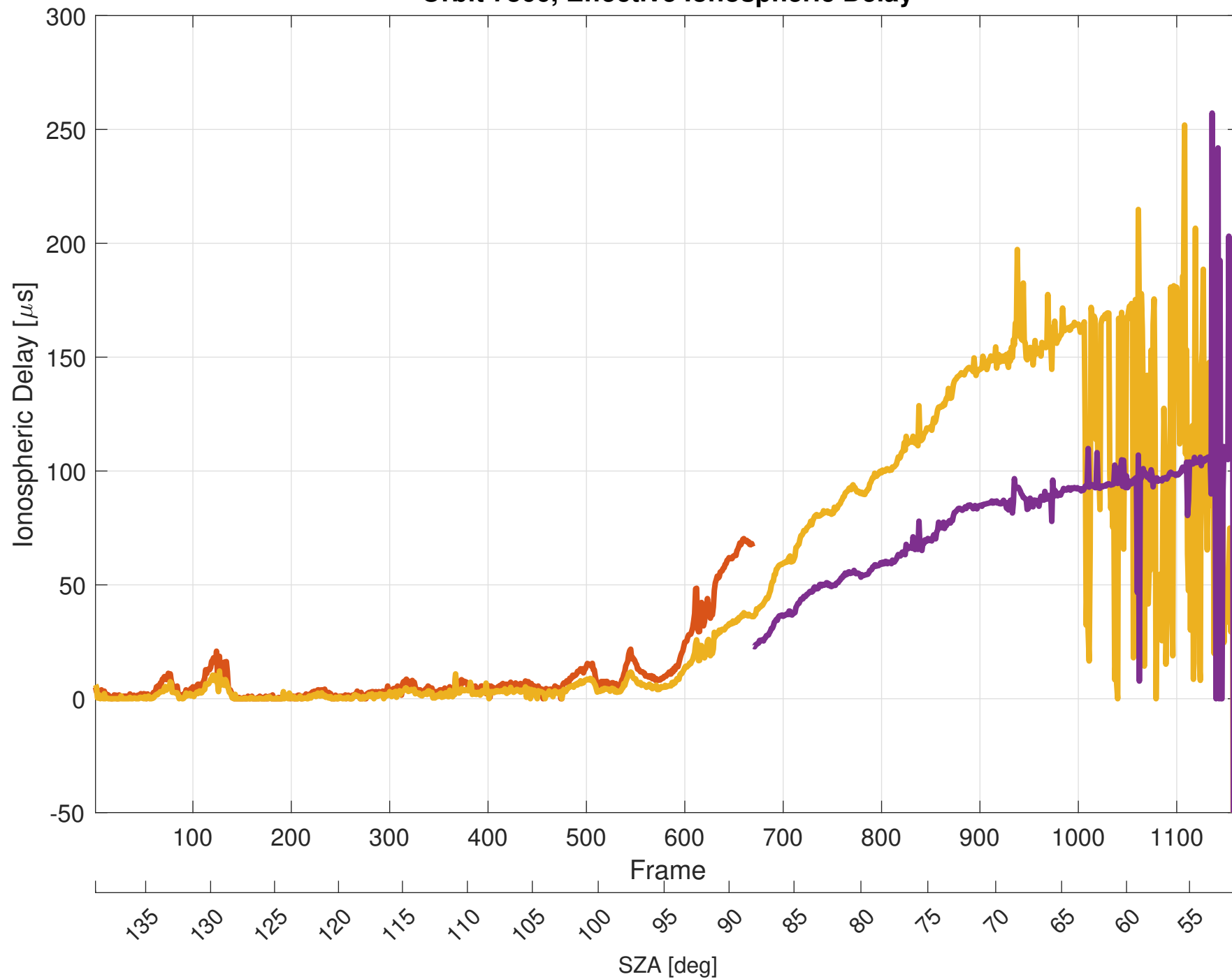
Orbit 7866, Effective Ionospheric Delay
