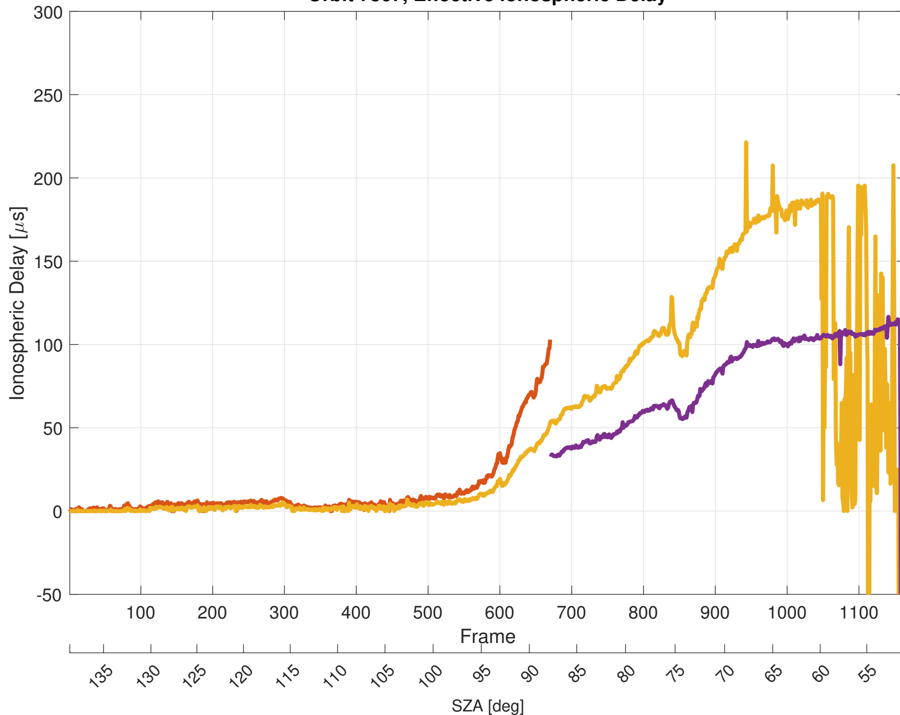
Orbit 7867, Effective Ionospheric Delay
