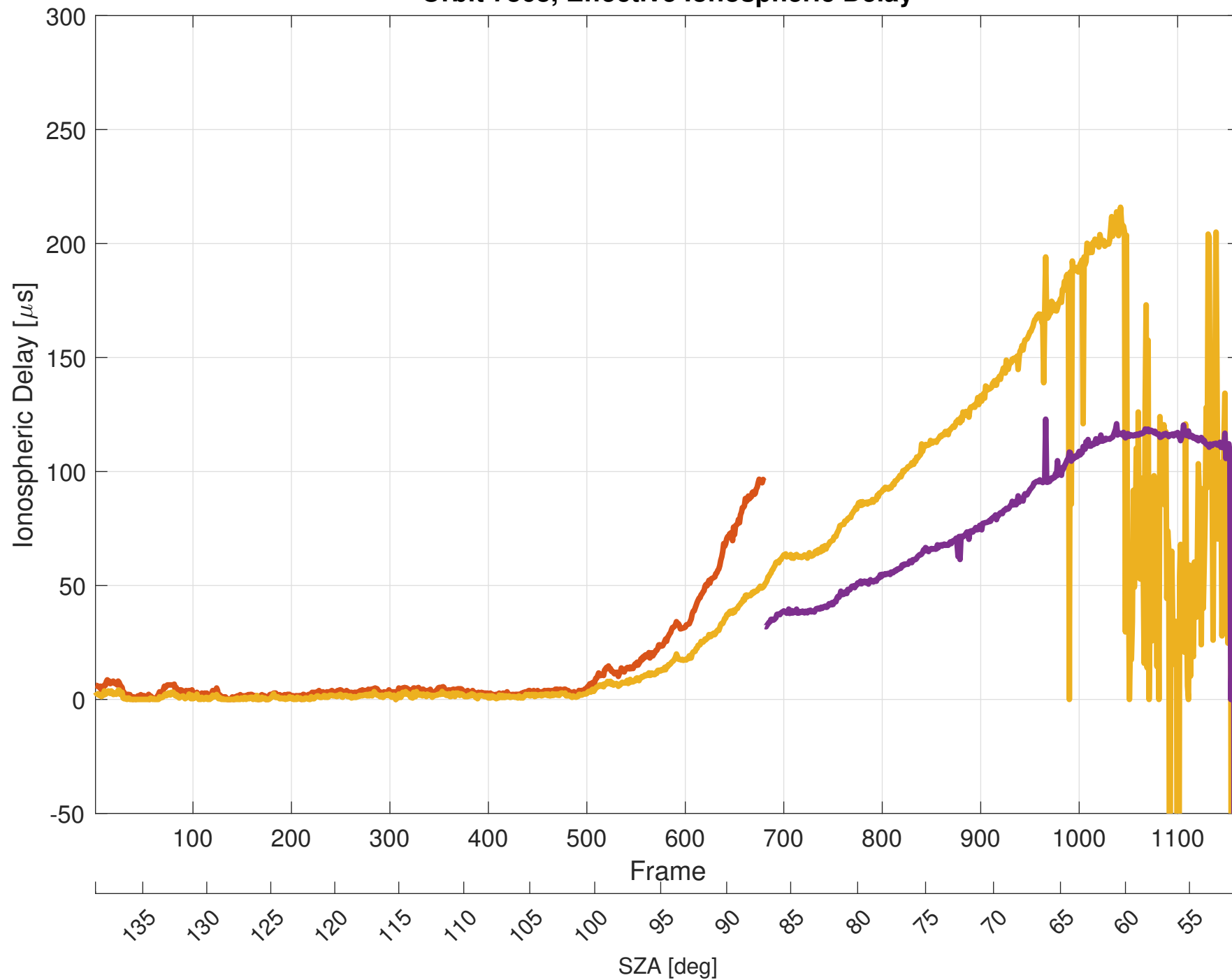
Orbit 7868, Effective Ionospheric Delay
