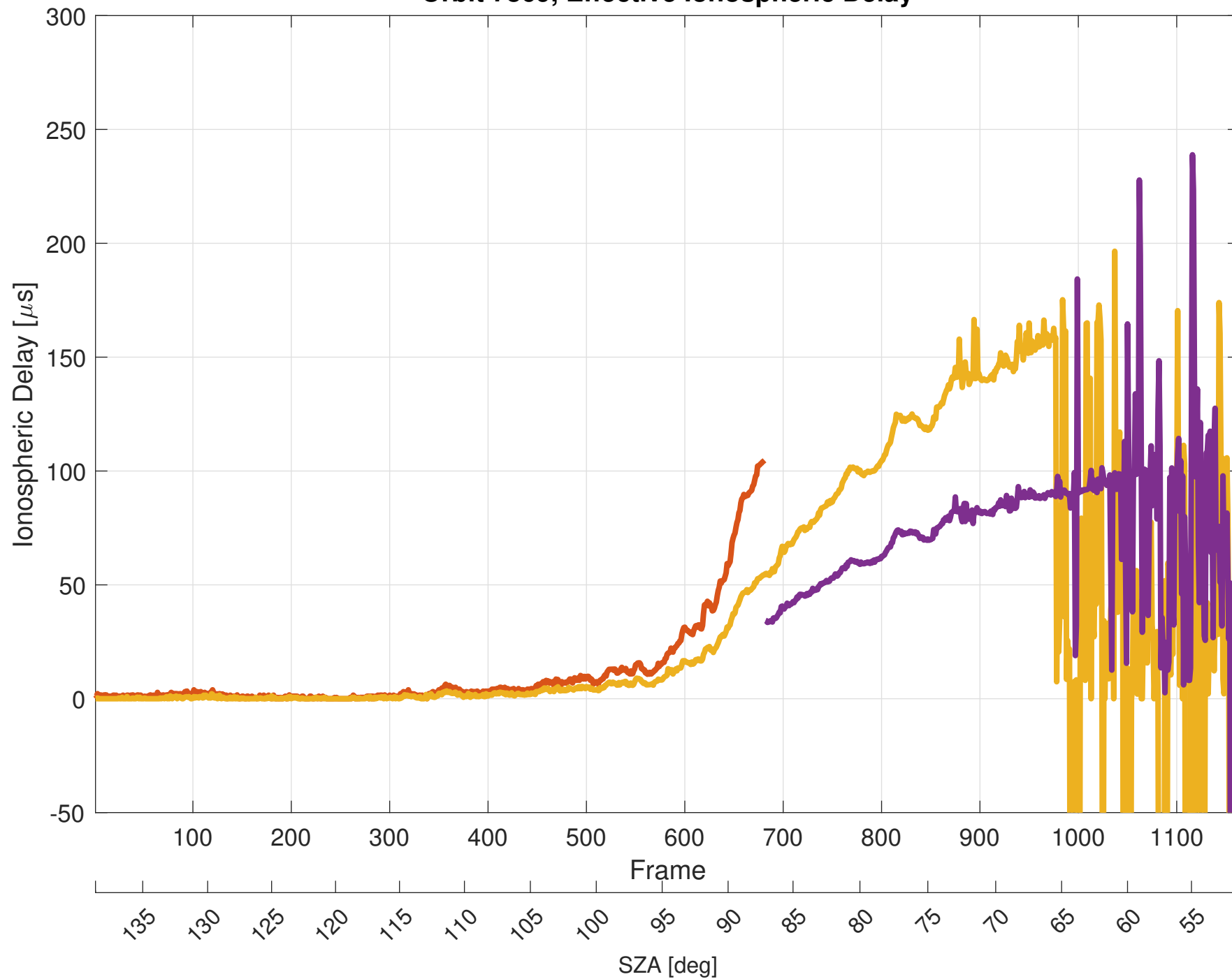
Orbit 7869, Effective Ionospheric Delay
