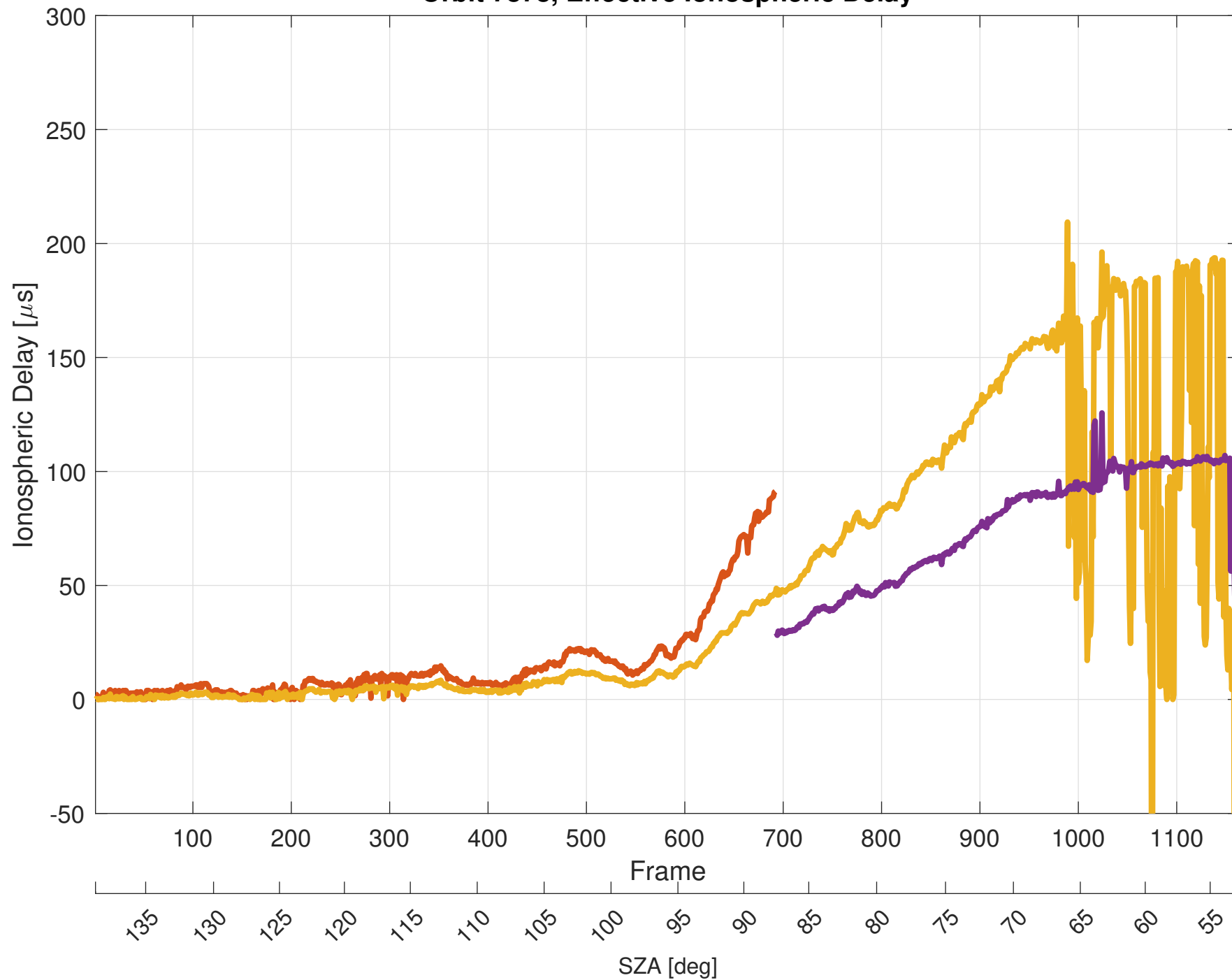
Orbit 7878, Effective Ionospheric Delay
