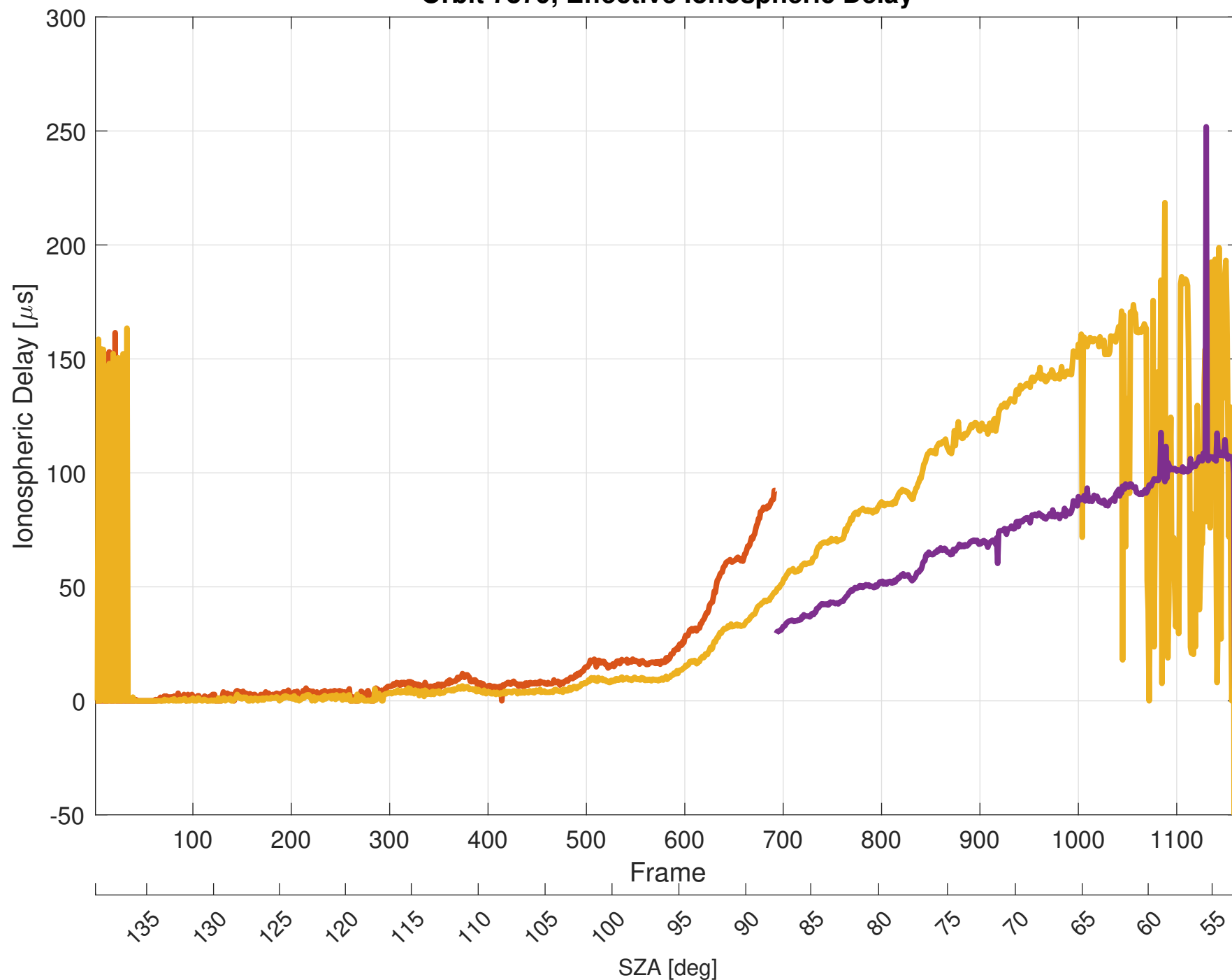
Orbit 7879, Effective Ionospheric Delay
